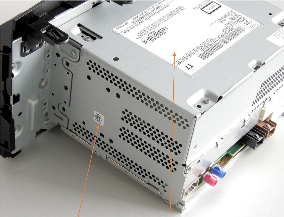
AIVIH61L0 with Draft labels: 1) Bosch label with Dot matrix code; 2) Customer label for displaying all necessary certification information (e.g. for FCC).
