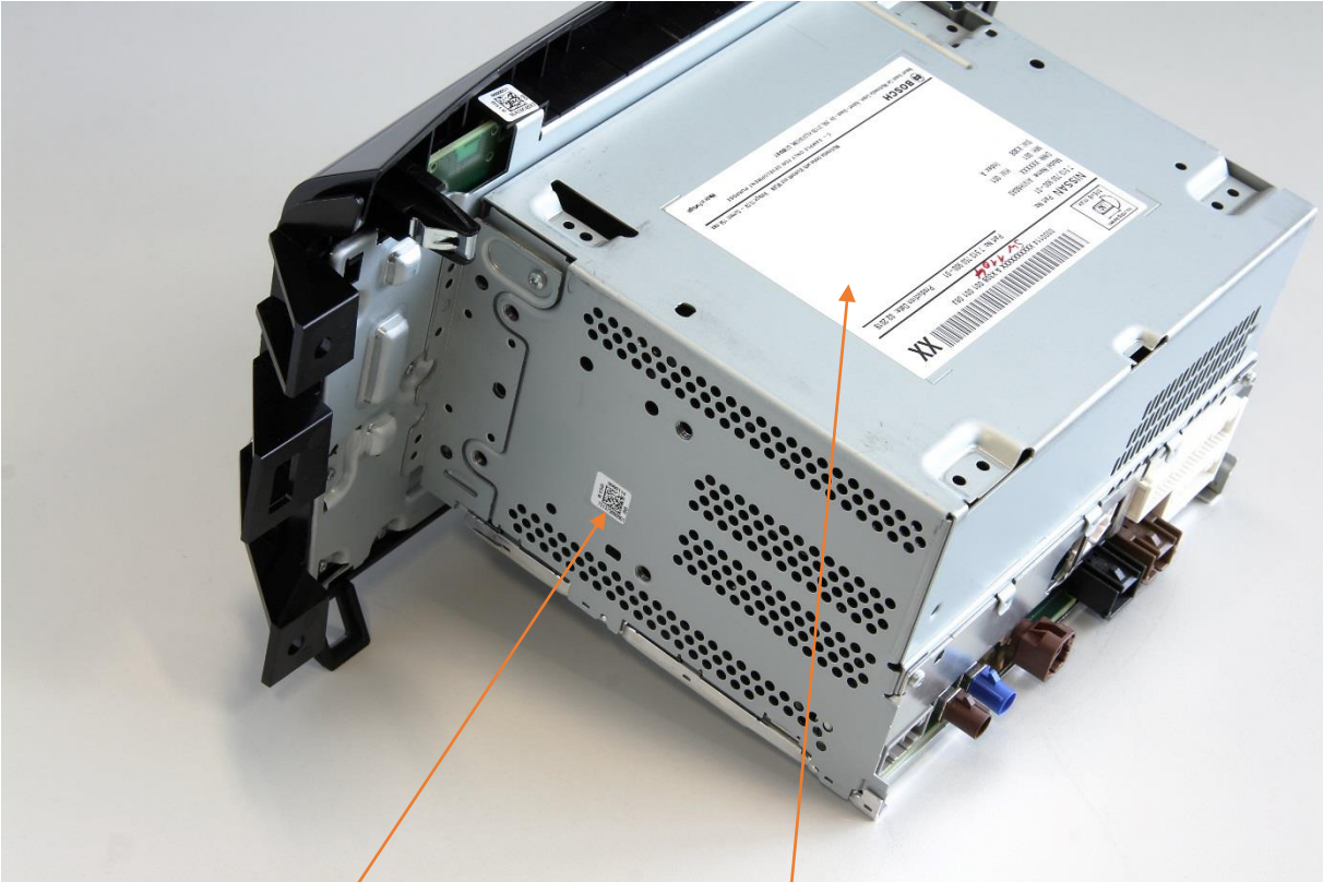
AIVIH60A0 with Draft labels: 1) Bosch label with Dot matrix code; 2) Customer label for displaying all necessary certification information (e.g. for FCC).
