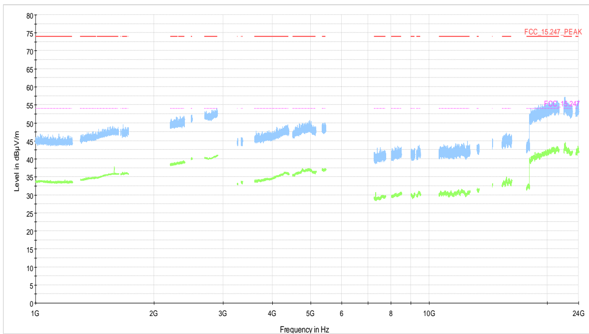
BT 8-DPSK (3-DH1) CH39
