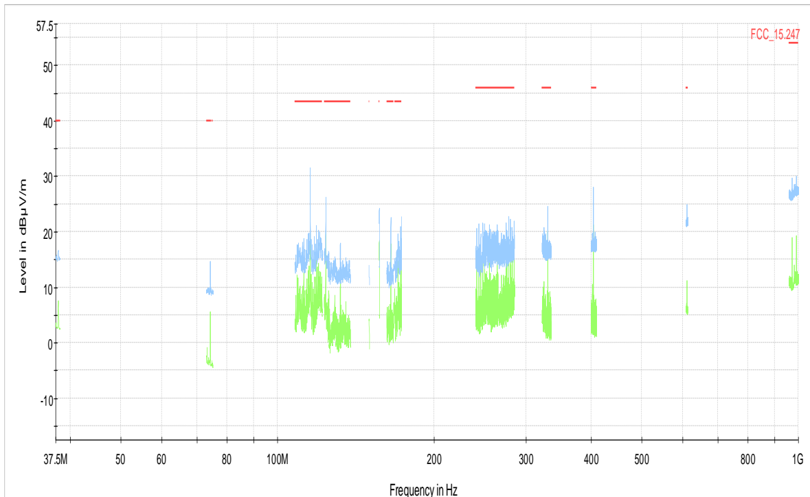
BT 8-DPSK (3-DH1) CH39
