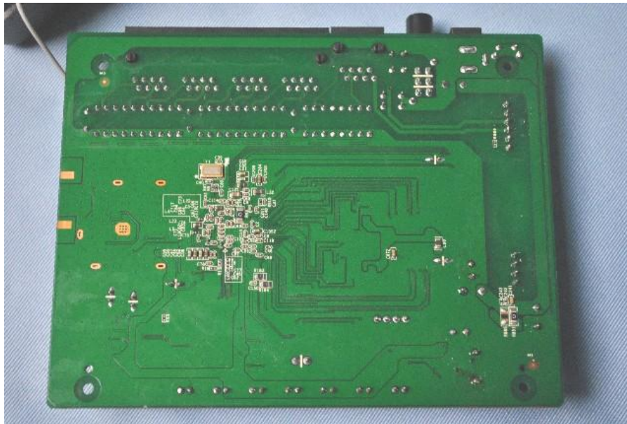
Main board solder side
