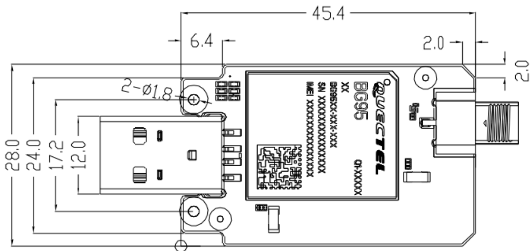
Figure 3.1: Topside view of QDM023-BG95-M1 communication module board
