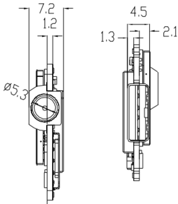
Figure 3.2: Side view of QDM023-BG95-M1 communication module board
