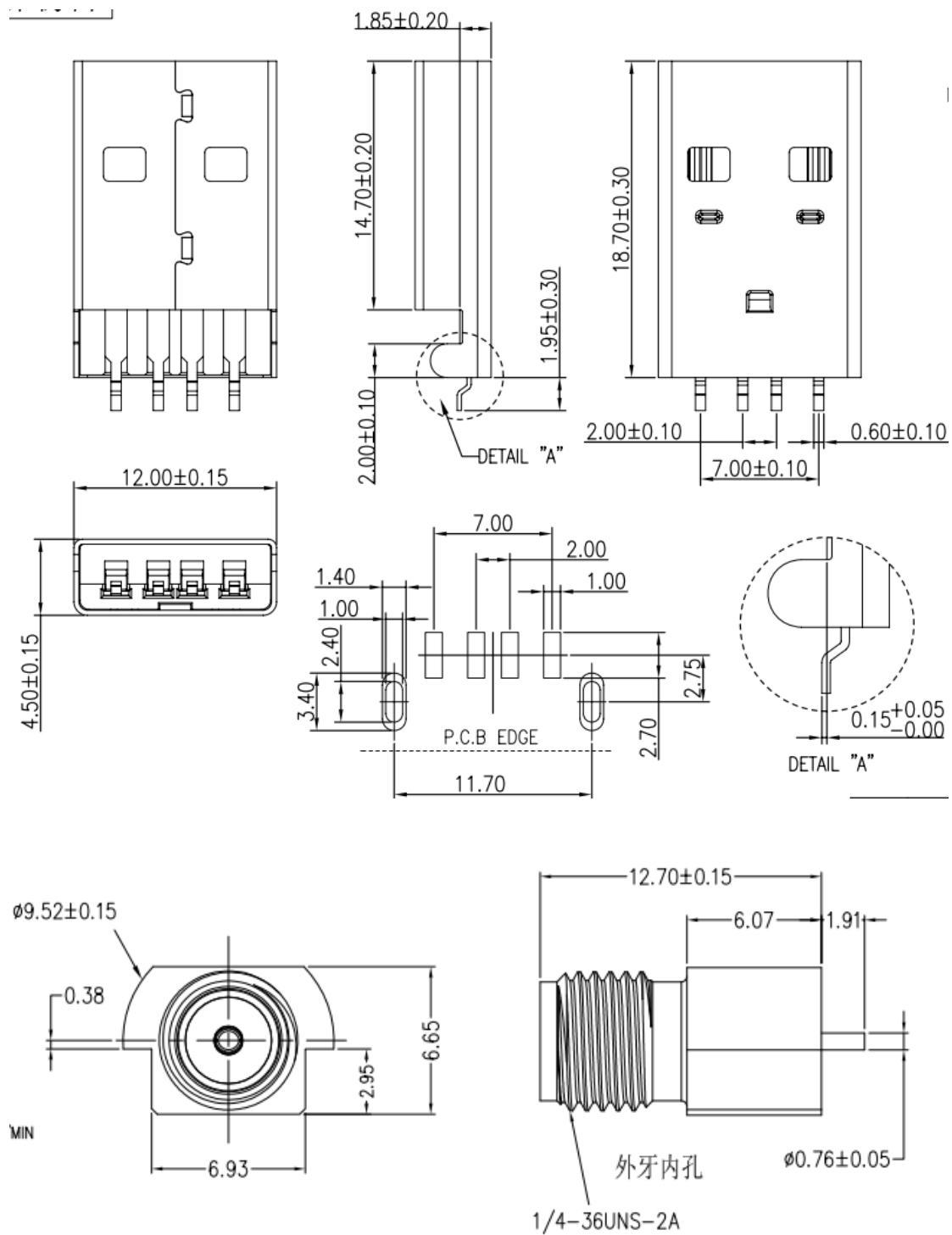
Figure 3-4: Mechanical dimensions of the connector
