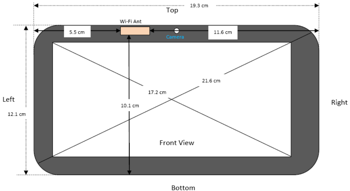
Fig.14.1 EUT Antenna Location
