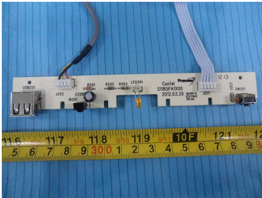
EUT – S1185PA1X00 Board Top View
