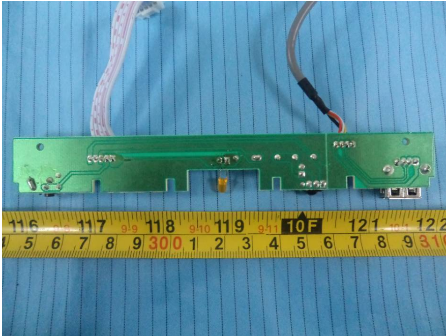
EUT – S1185PA1X00 Board Bottom View
