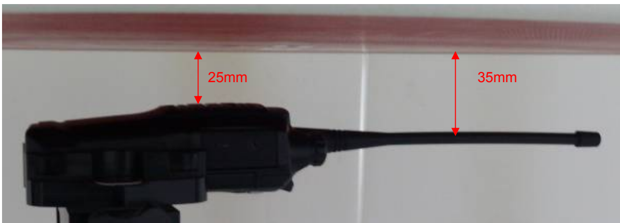
Picture 4: Face-held, the front of the EUT towards phantom, the distance from the EUT Antenna to the bottom of the Phantom is 35mm
