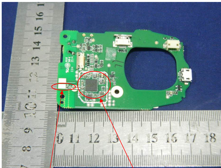
Antenna Contact 1
