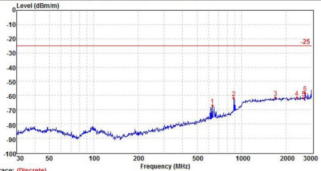
Trace: (Discrete)
