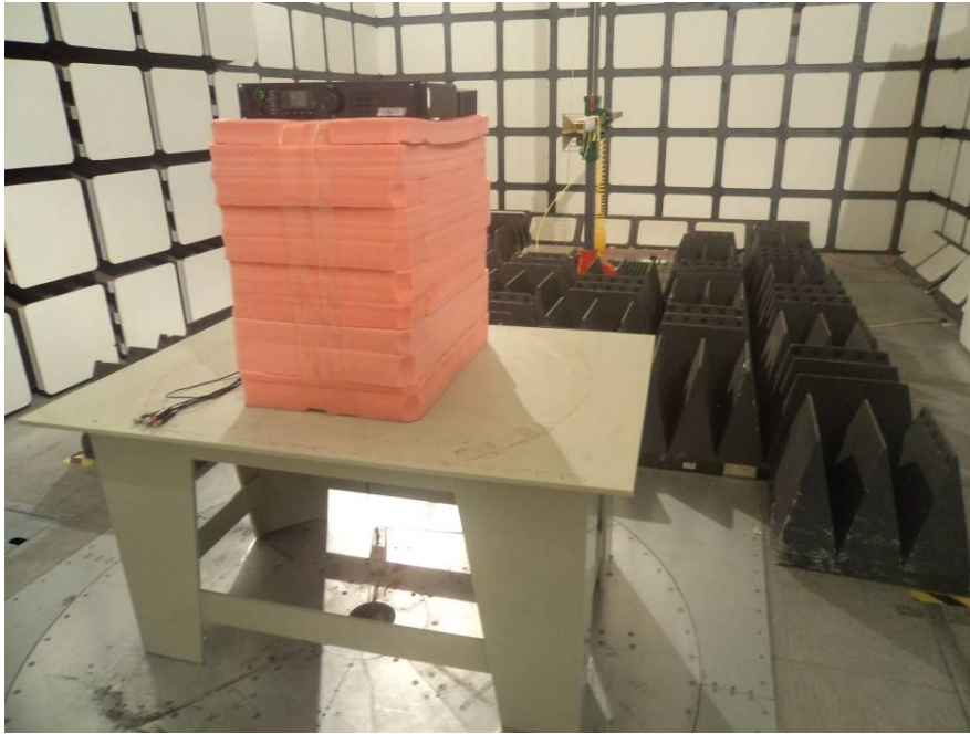
Above 1 GHz: Transmitting Radiated Emissions – Front View
