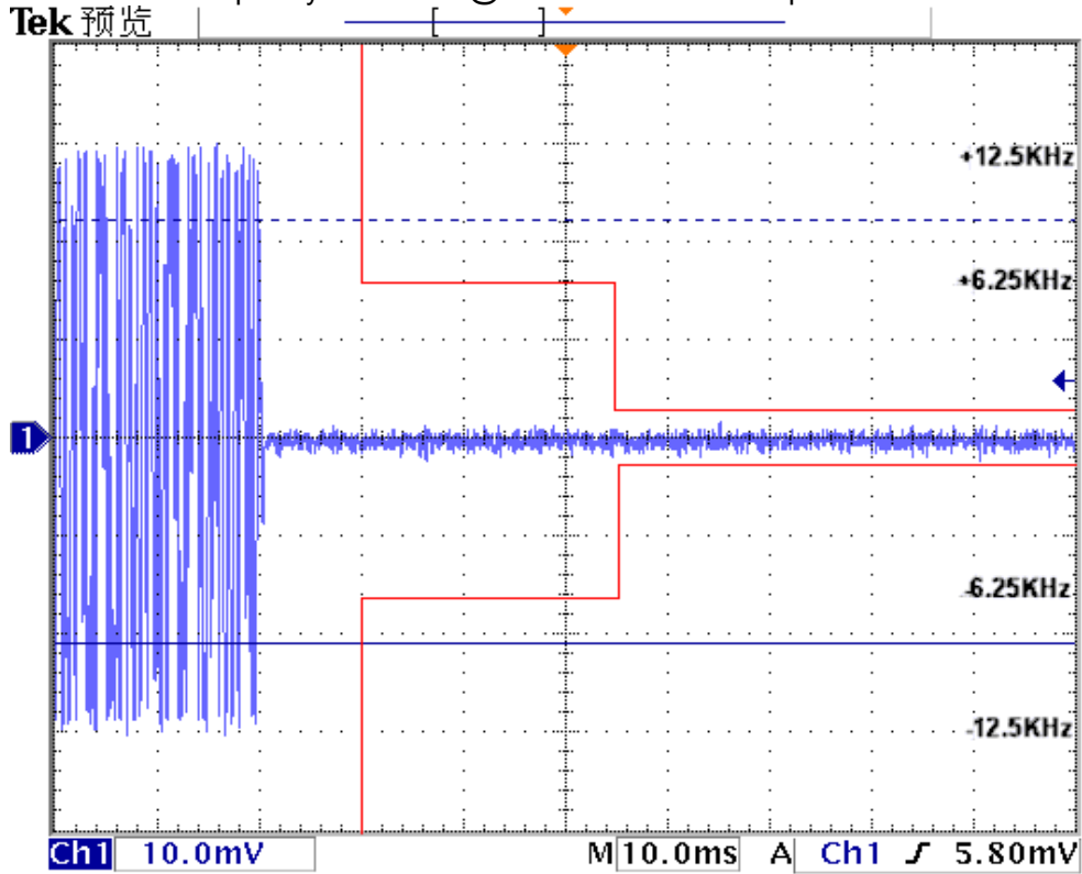
Transmitter Frequency Behaviour @ 12.5 KHz Channel Separation-----Off – On
