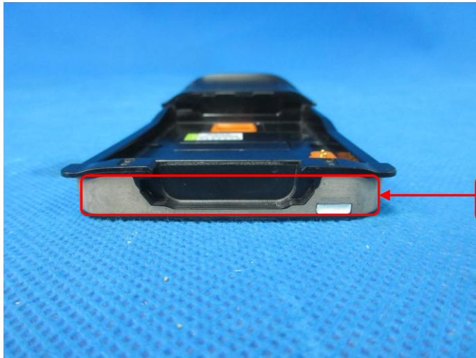
2G/3G/4G ANT
