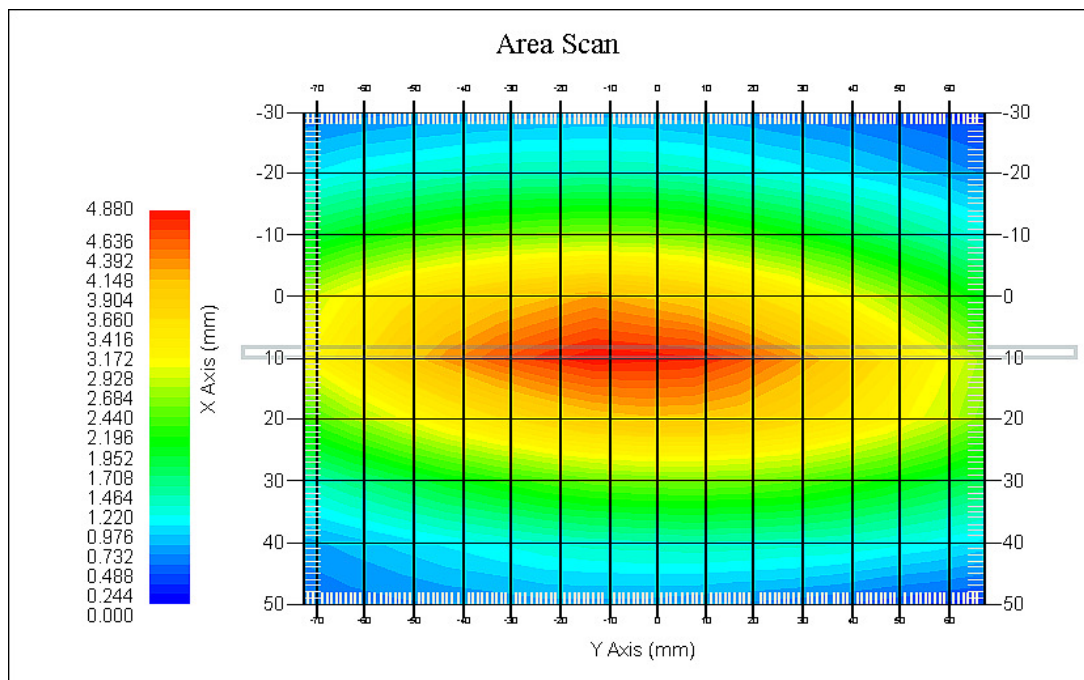
450 MHz System Validation with Head Tissue
