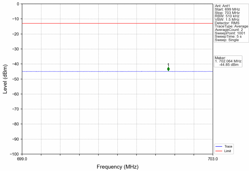
n71_15kHz_SISO_NTNV_20MHz_CP-OFDM QPSK_680.5MHz_Edge_1RB_Left
