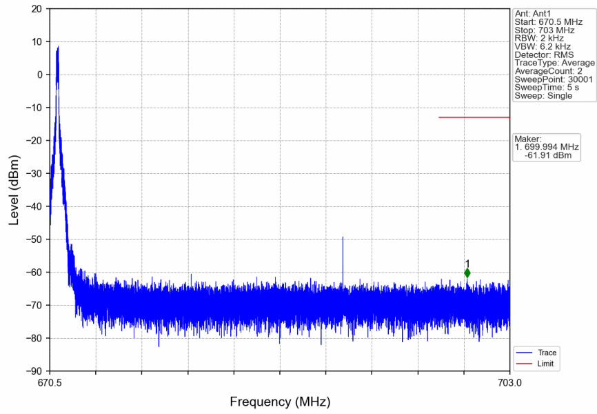
n71_15kHz_SISO_NTNV_20MHz_CP-OFDM QPSK_680.5MHz_Edge_1RB_Left
