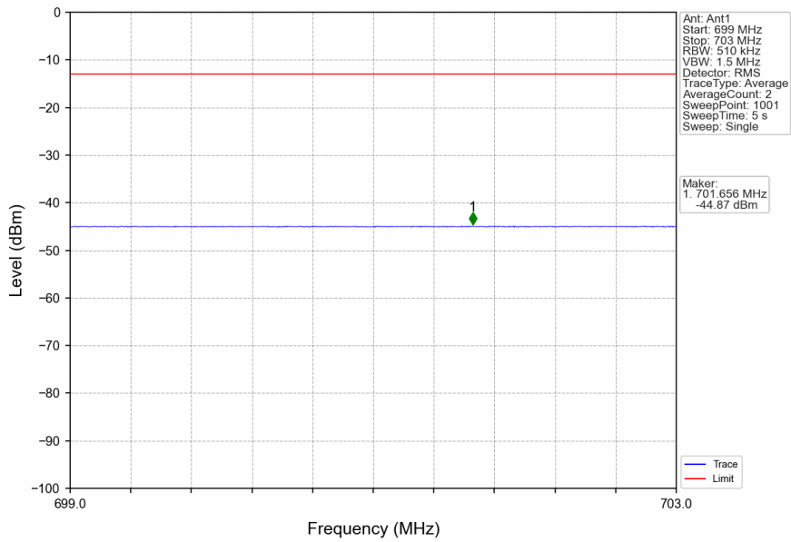
n71_15kHz_SISO_NTNV_15MHz_CP-OFDM_QPSK_680.5MHz_Edge_1RB_Left
