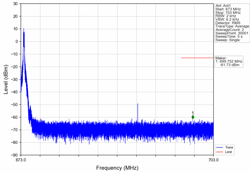
n71_15kHz_SISO_NTNV_15MHz_CP-OFDM_QPSK_680.5MHz_Edge_1RB_Left
