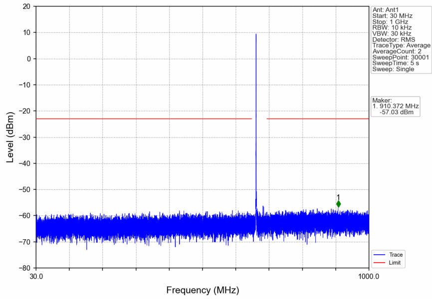
n71_15kHz_SISO_NTNV_20MHz_DFT-s-OFDM QPSK_680.5MHz_Edge_1RB_Left
