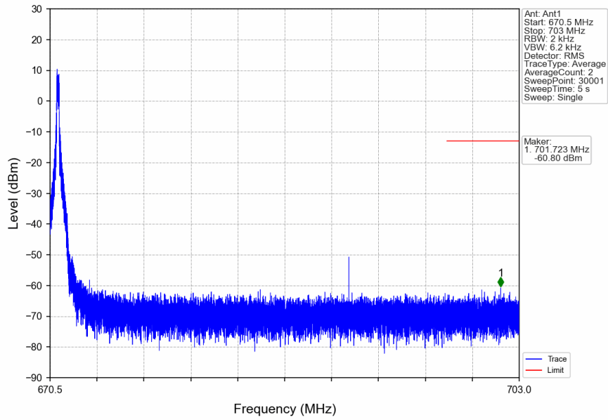
n71_15kHz_SISO_NTNV_20MHz_DFT-s-OFDM QPSK_680.5MHz_Edge_1RB_Left
