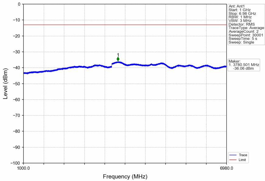
n71_15kHz_SISO_NTNV_20MHz_DFT-s-OFDM QPSK_680.5MHz_Edge_1RB_Left
