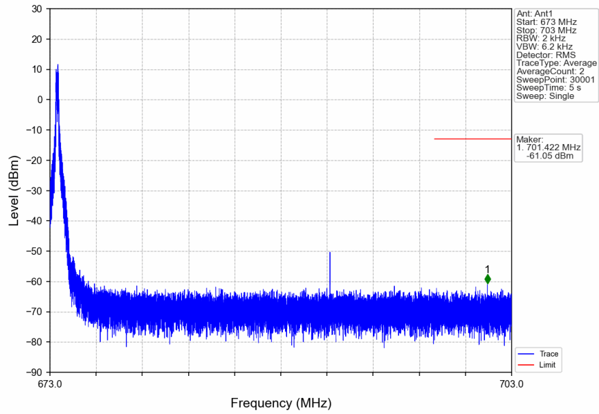
n71_15kHz_SISO_NTNV_15MHz_DFT-s-OFDM QPSK_680.5MHz_Edge_1RB_Left
