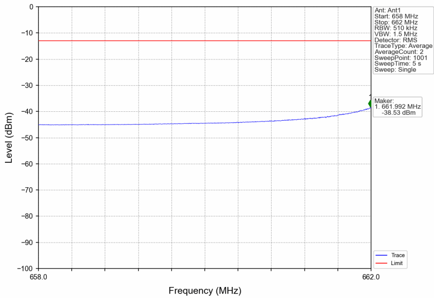
n71_15kHz_SISO_NTNV_15MHz_DFT-s-OFDM QPSK_670.5MHz_Edge_1RB_Left
