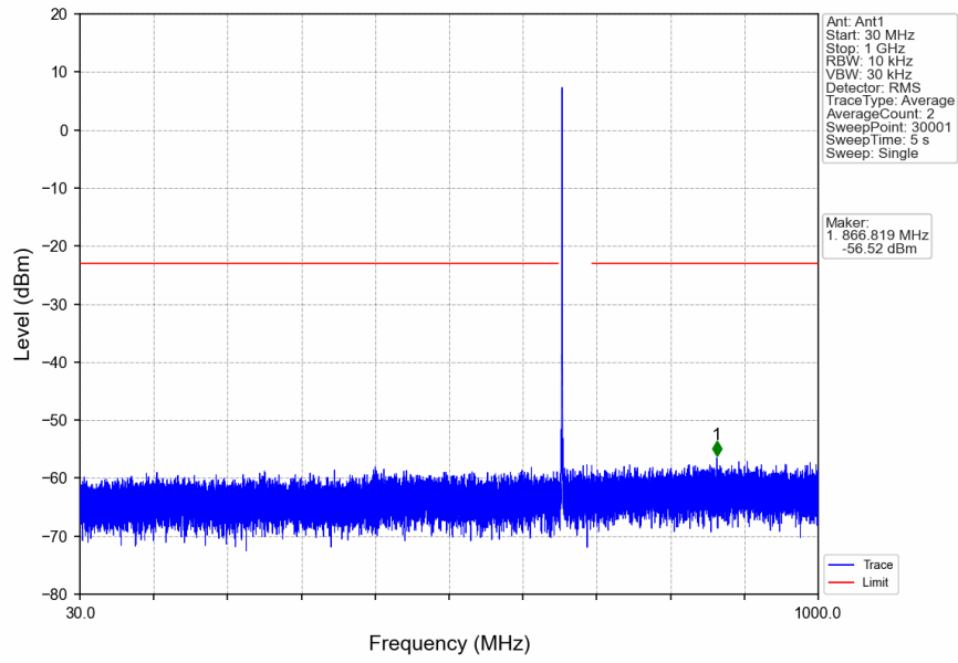
n71_15kHz_SISO_NTNV_15MHz_CP-OFDM QPSK_670.5MHz_Edge_1RB_Left
