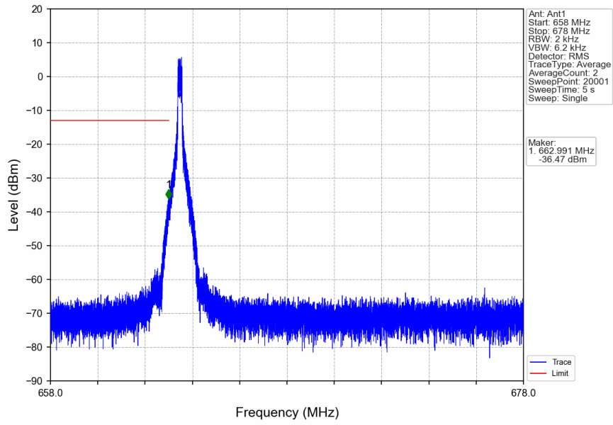
n71_15kHz_SISO_NTNV_15MHz_DFT-s-OFDM QPSK_670.5MHz_Edge_1RB_Left
