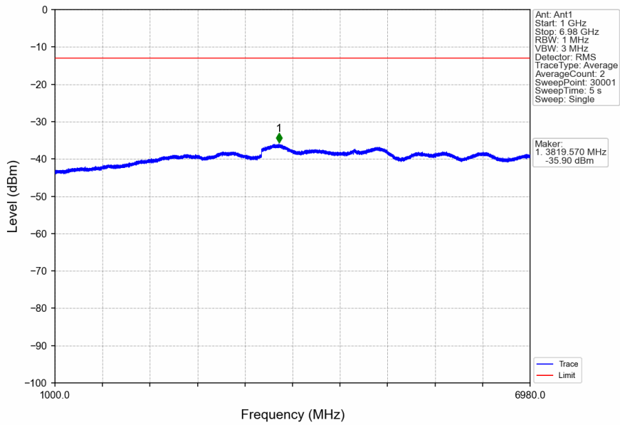
n71_15kHz_SISO_NTNV_15MHz_DFT-s-OFDM QPSK_680.5MHz_Edge_1RB_Left
