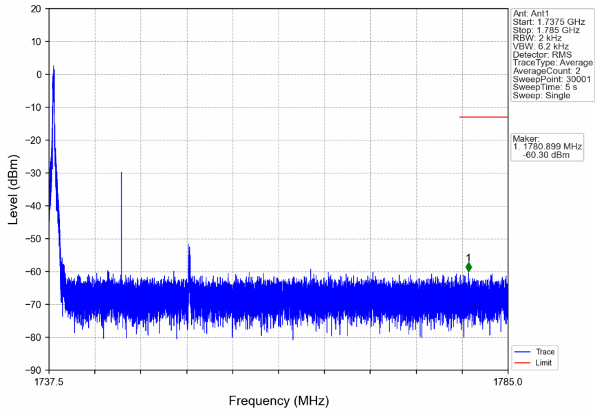
n66_15kHz_SISO_NTNV_15MHz_CP-OFDM QPSK_1745MHz_Edge_1RB_Left
