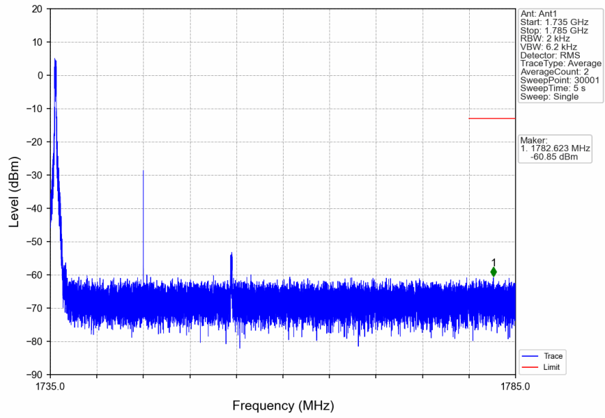
n66_15kHz_SISO_NTNV_20MHz_DFT-s-OFDM QPSK_1745MHz_Edge_1RB_Left
