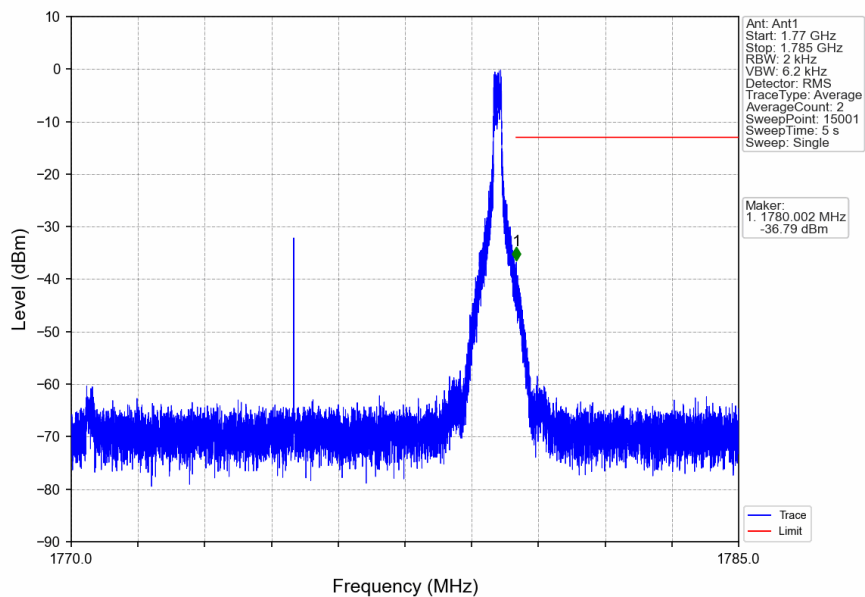
n66_15kHz_SISO_NTNV_10MHz_CP-OFDM QPSK_1775MHz_Edge_1RB_Right
