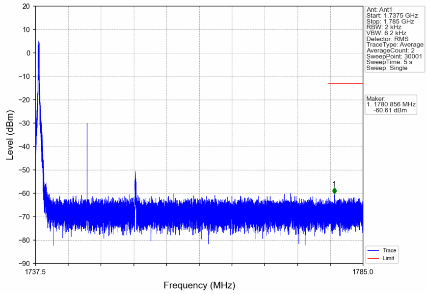
n66_15kHz_SISO_NTNV_15MHz_DFT-s-OFDM_QPSK_1745MHz_Edge_1RB_Left
