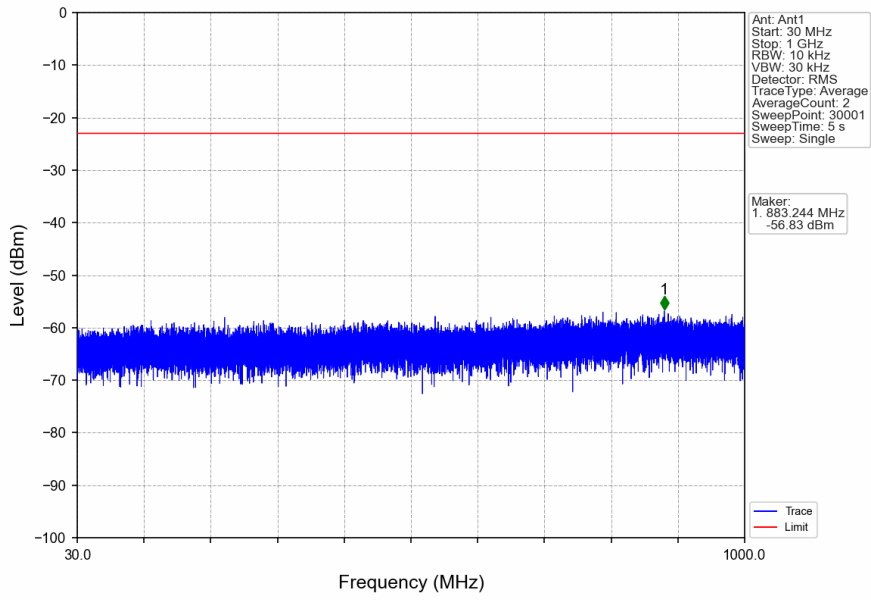
n66_15kHz_SISO_NTNV_15MHz_CP-OFDM QPSK_1717.5MHz_Edge_1RB_Left
