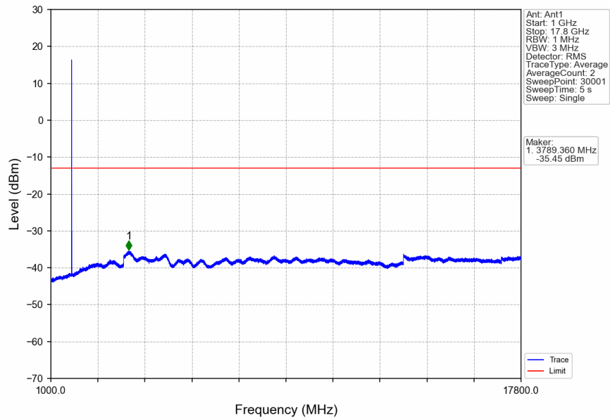
n66_15kHz_SISO_NTNV_15MHz_DFT-s-OFDM_QPSK_1745MHz_Edge_1RB_Left
