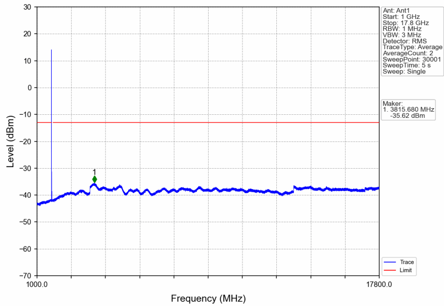
n66_15kHz_SISO_NTNV_15MHz_CP-OFDM QPSK_1717.5MHz_Edge_1RB_Left
