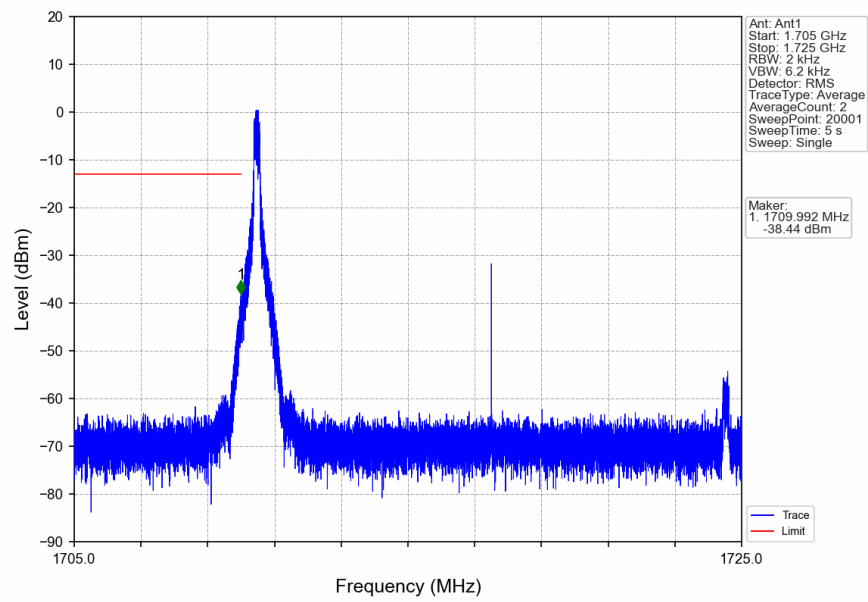
n66_15kHz_SISO_NTNV_15MHz_CP-OFDM QPSK_1717.5MHz_Edge_1RB_Left
