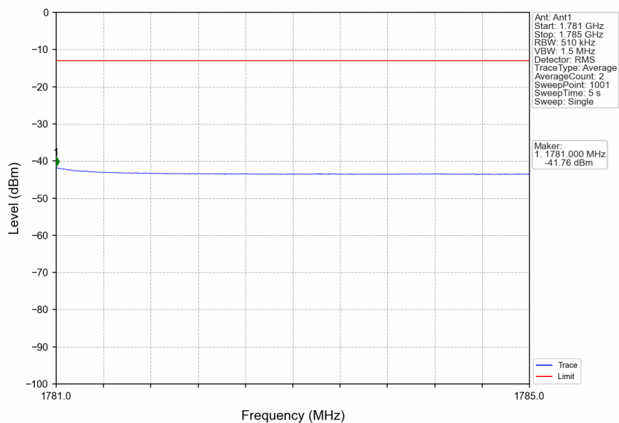
n66_15kHz_SISO_NTNV_10MHz_CP-OFDM QPSK_1775MHz_Edge_1RB_Right
