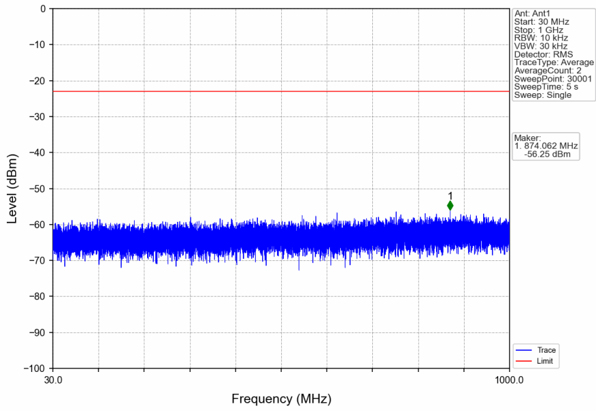
n66_15kHz_SISO_NTNV_15MHz_DFT-s-OFDM_QPSK_1745MHz_Edge_1RB_Left
