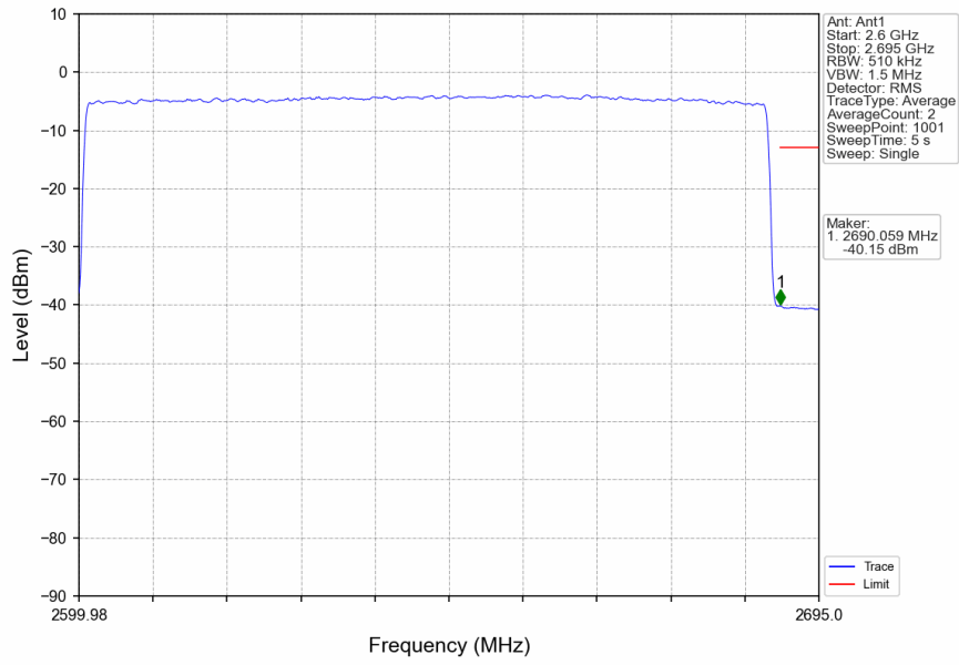
n41_30kHz_SISO_NTNV_90MHz_DFT-s-OFDM QPSK_2644.98MHz_Outer_Full
