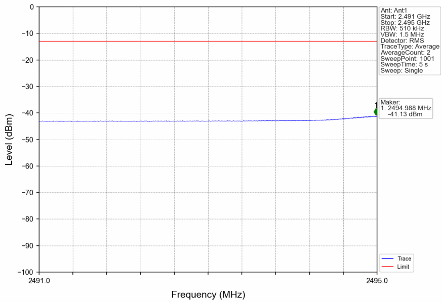
n41_30kHz_SISO_NTNV_100MHz_DFT-s-OFDM QPSK_2546.01MHz_Edge_1RB_Left
