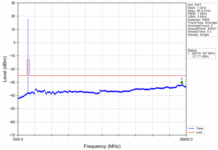
n41_30kHz_SISO_NTNV_90MHz_CP-OFDM QPSK_2592.99MHz_Edge_1RB_Left
