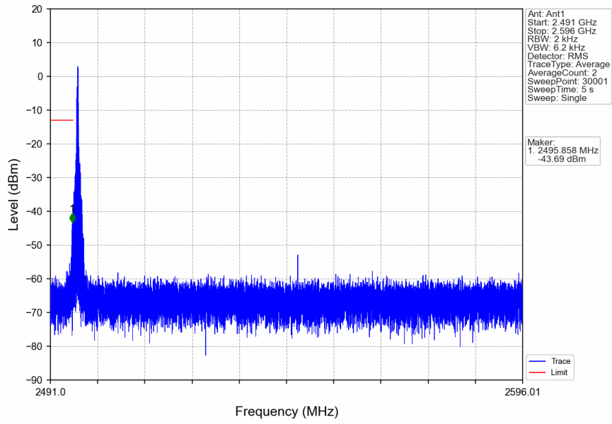
n41_30kHz_SISO_NTNV_100MHz_DFT-s-OFDM QPSK_2546.01MHz_Edge_1RB_Left
