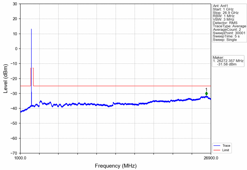
n41_30kHz_SISO_NTNV_80MHz_CP-OFDM_QPSK_2536.02MHz_Edge_1RB_Left
