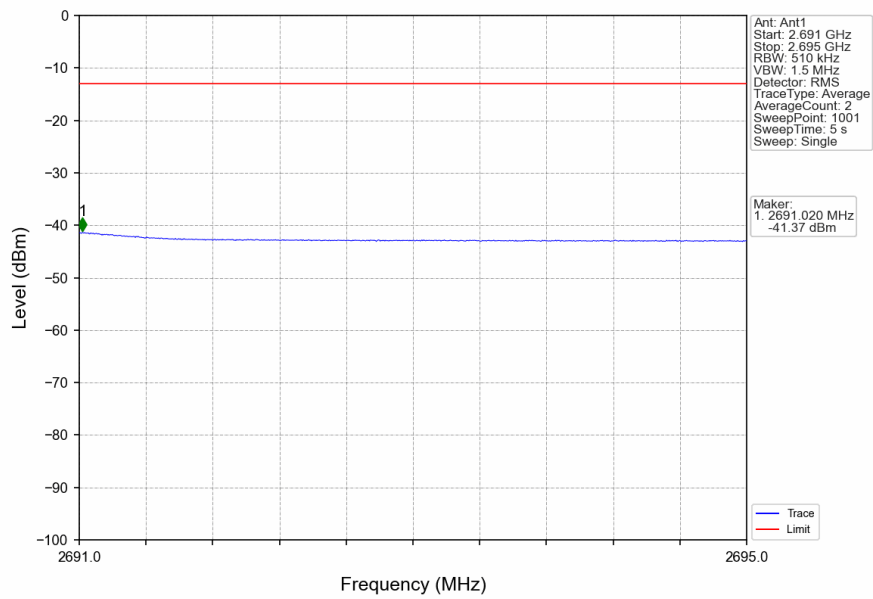
n41_30kHz_SISO_NTNV_80MHz_CP-OFDM QPSK_2649.99MHz_Edge_1RB_Right
