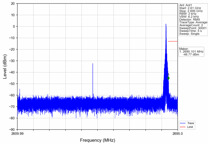
n41_30kHz_SISO_NTNV_80MHz_CP-OFDM QPSK_2649.99MHz_Edge_1RB_Right
