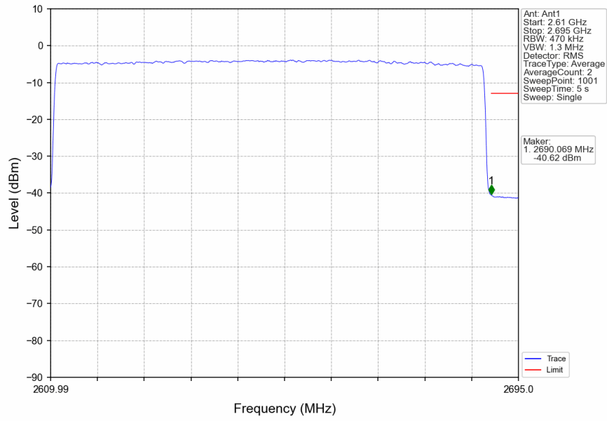
n41_30kHz_SISO_NTNV_80MHz_DFT-s-OFDM QPSK_2649.99MHz_Outer_Full
