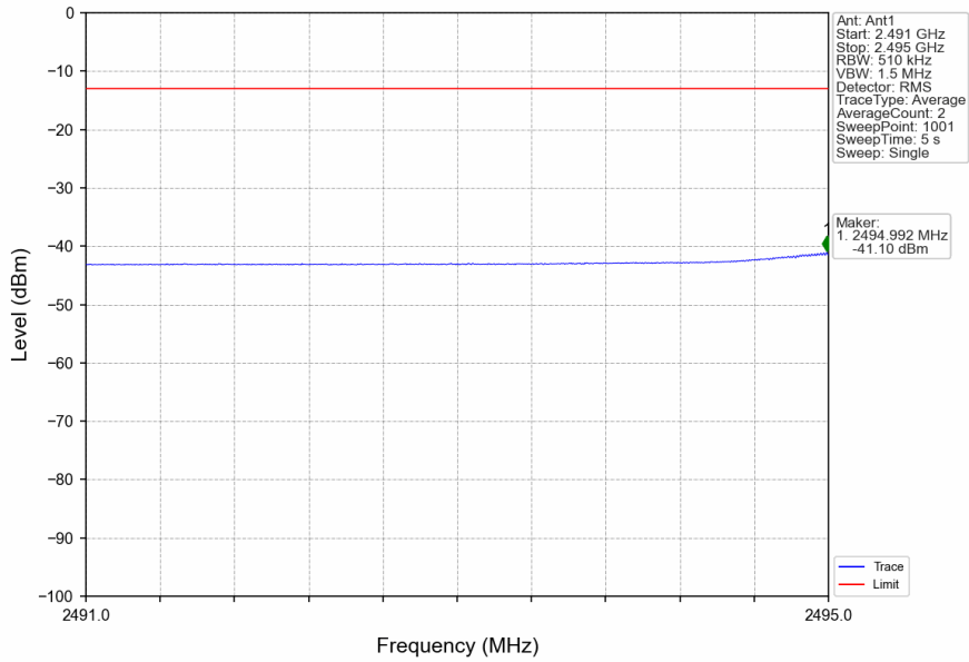
n41_30kHz_SISO_NTNV_80MHz_CP-OFDM_QPSK_2536.02MHz_Edge_1RB_Left
