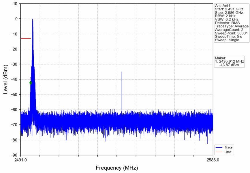
n41_30kHz_SISO_NTNV_90MHz_DFT-s-OFDM_QPSK_2541MHz_Edge_1RB_Left
