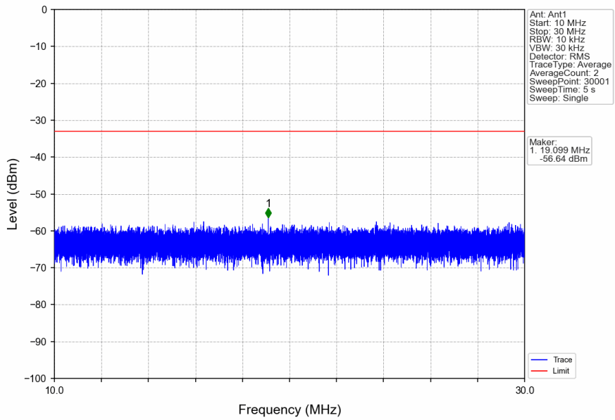
n41_30kHz_SISO_NTNV_90MHz_DFT-s-OFDM_QPSK_2541MHz_Edge_1RB_Left
