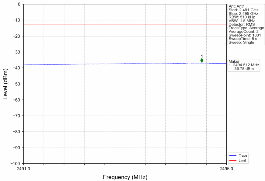
n41_30kHz_SISO_NTNV_60MHz_CP-OFDM QPSK_2526MHz_Outer_Full
