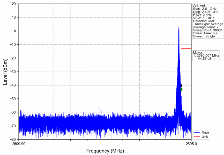
n41_30kHz_SISO_NTNV_80MHz_DFT-s-OFDM PI/2 BPSK_2649.99MHz_Edge_1RB_Right
