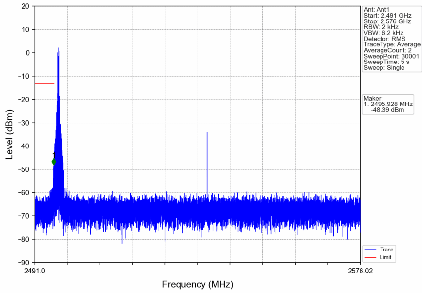
n41_30kHz_SISO_NTNV_80MHz_DFT-s-OFDM QPSK_2536.02MHz_Edge_1RB_Left
