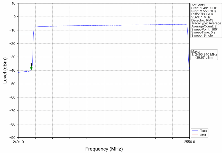
n41_30kHz_SISO_NTNV_60MHz_CP-OFDM QPSK_2526MHz_Outer_Full
