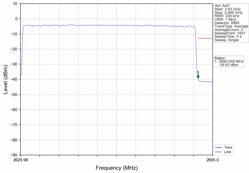
n41_30kHz_SISO_NTNV_60MHz_DFT-s-OFDM_QPSK_2659.98MHz_Outer_Full
