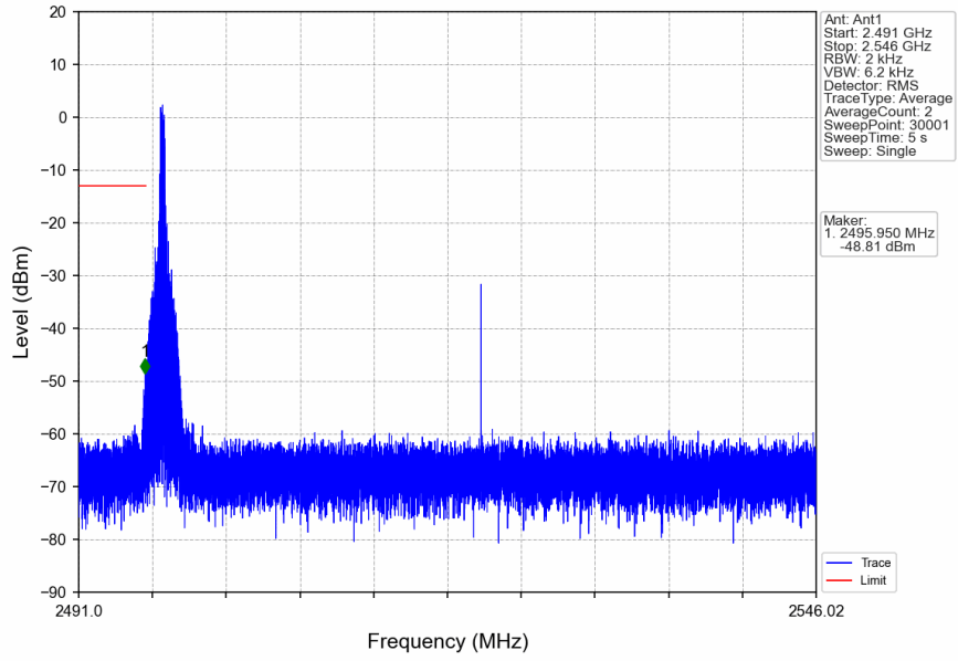
n41_30kHz_SISO_NTNV_50MHz_CP-OFDM QPSK_2521.02MHz_Edge_1RB_Left
