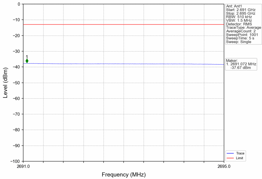
n41_30kHz_SISO_NTNV_60MHz_DFT-s-OFDM_QPSK_2659.98MHz_Outer_Full
