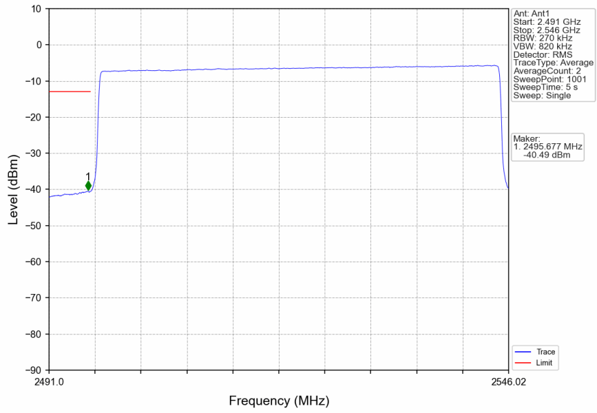
n41_30kHz_SISO_NTNV_50MHz_CP-OFDM QPSK_2521.02MHz_Outer_Full
