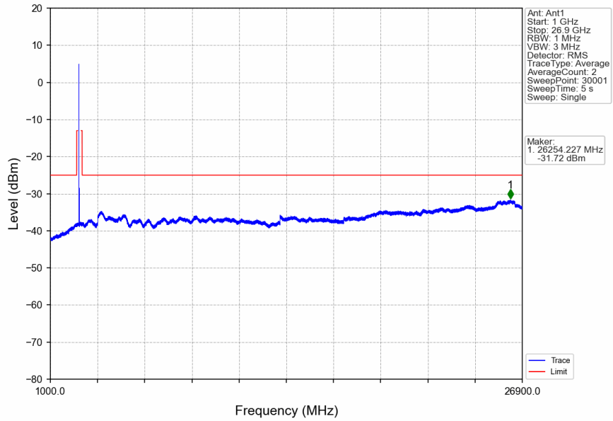
n41_30kHz_SISO_NTNV_50MHz_CP-OFDM QPSK_2592.99MHz_Edge_1RB_Left
