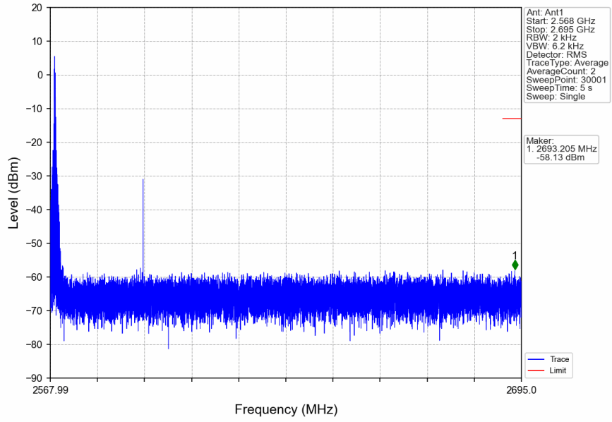
n41_30kHz_SISO_NTNV_50MHz_CP-OFDM QPSK_2592.99MHz_Edge_1RB_Left
