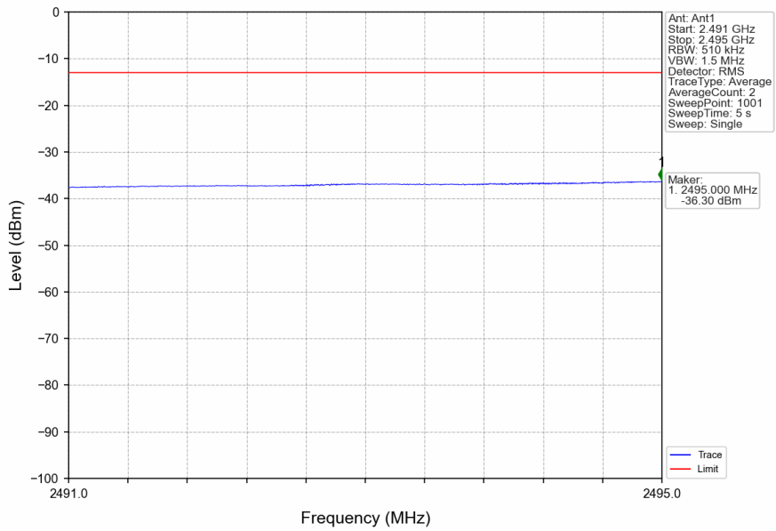
n41_30kHz_SISO_NTNV_50MHz_CP-OFDM QPSK_2521.02MHz_Outer_Full
