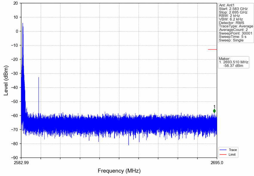
n41_30kHz_SISO_NTNV_20MHz_CP-OFDM_QPSK_2592.99MHz_Edge_1RB_Left
