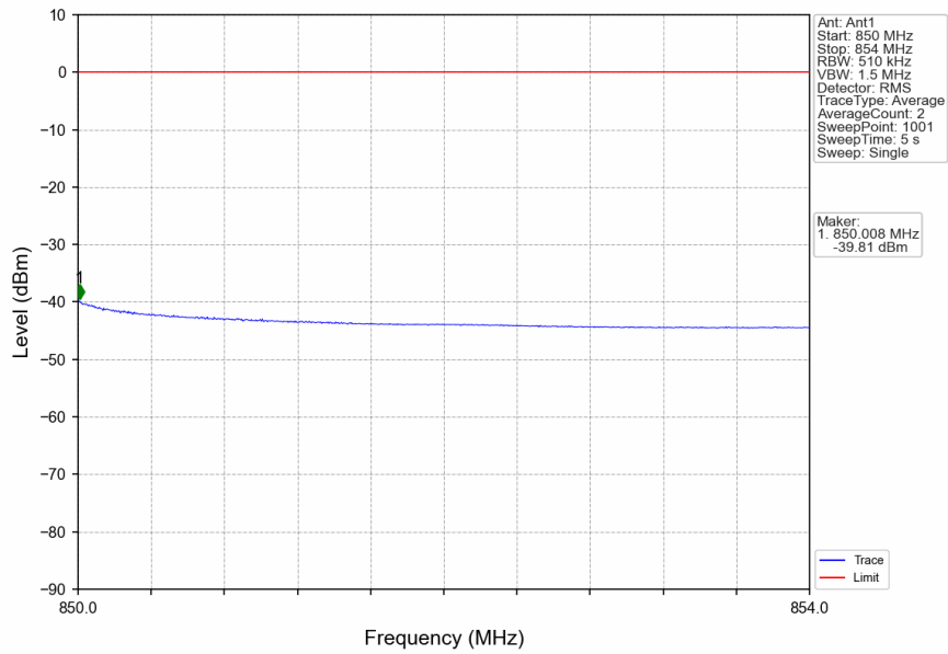
n5_15kHz_SISO_NTNV_20MHz_CP-OFDM QPSK_839MHz_Edge_1RB_Right
