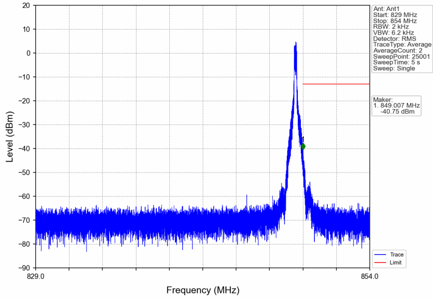
n5_15kHz_SISO_NTNV_20MHz_CP-OFDM QPSK_839MHz_Edge_1RB_Right
