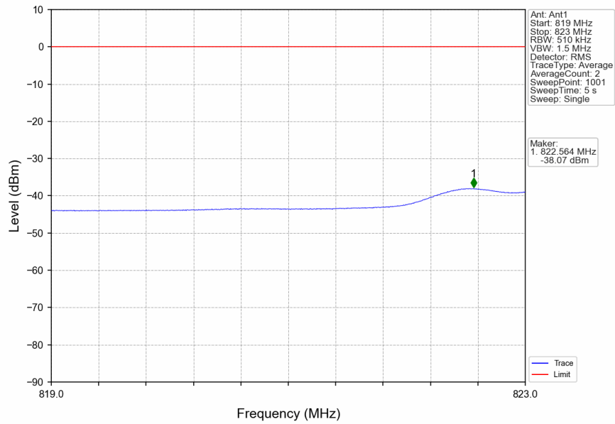
n5_15kHz_SISO_NTNV_5MHz_DFT-s-OFDM QPSK_826.5MHz_Inner_1RB_Left
