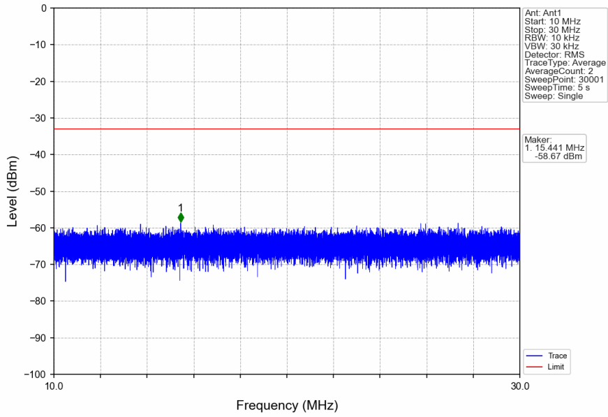
n5_15kHz_SISO_NTNV_5MHz_CP-OFDM QPSK_836.5MHz_Edge_1RB_Left
