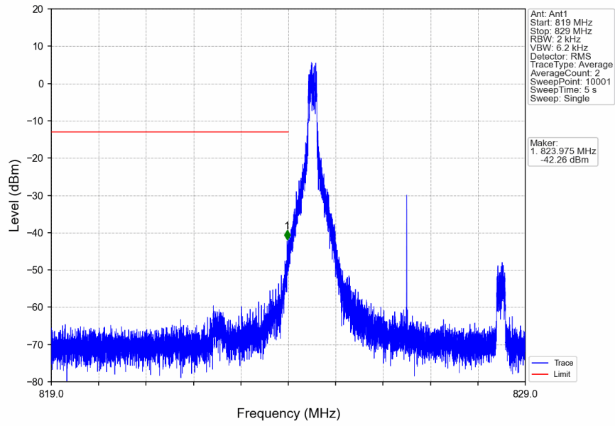
n5_15kHz_SISO_NTNV_5MHz_DFT-s-OFDM QPSK_826.5MHz_Inner_1RB_Left
