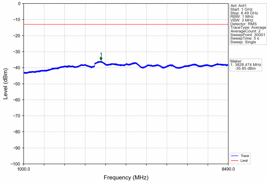
n5_15kHz_SISO_NTNV_5MHz_CP-OFDM QPSK_826.5MHz_Edge_1RB_Left
