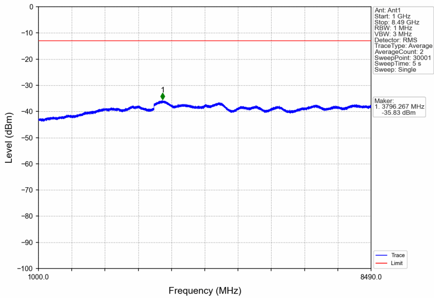
n5_15kHz_SISO_NTNV_5MHz_DFT-s-OFDM QPSK_826.5MHz_Edge_1RB_Left
