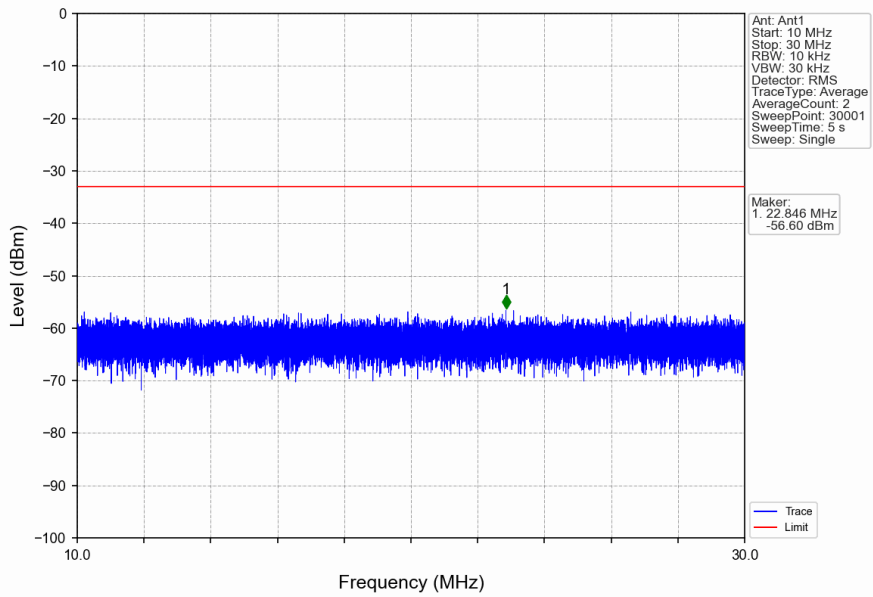
n5_15kHz_SISO_NTNV_5MHz_DFT-s-OFDM PI/2 BPSK_836.5MHz_Edge_1RB_Left
