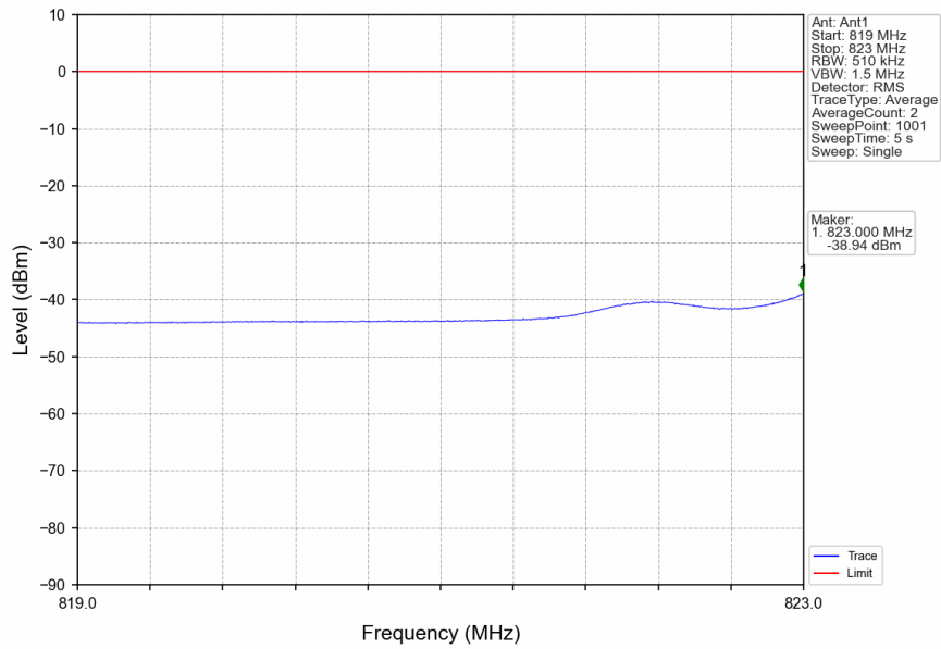
n5_15kHz_SISO_NTNV_5MHz_CP-OFDM QPSK_826.5MHz_Edge_1RB_Left
