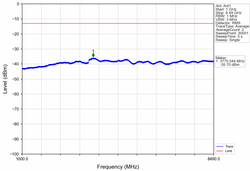
n5_15kHz_SISO_NTNV_5MHz_DFT-s-OFDM QPSK_836.5MHz_Edge_1RB_Left
