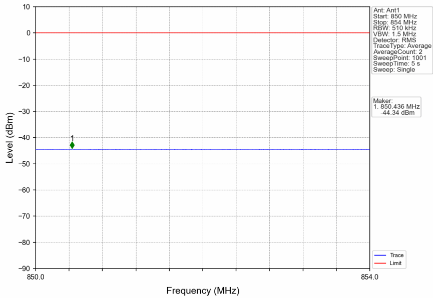
n5_15kHz_SISO_NTNV_5MHz_CP-OFDM QPSK_836.5MHz_Edge_1RB_Left
