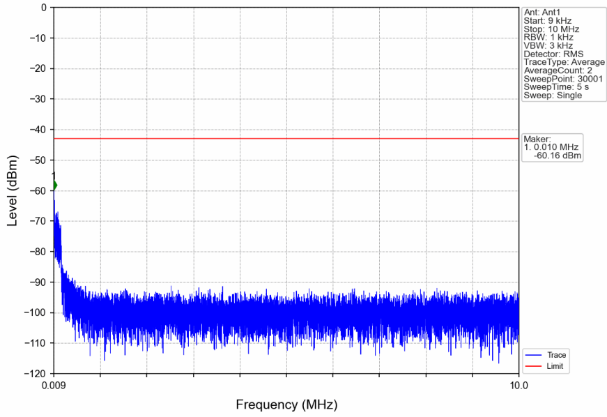
n5_15kHz_SISO_NTNV_5MHz_DFT-s-OFDM QPSK_836.5MHz_Edge_1RB_Left
