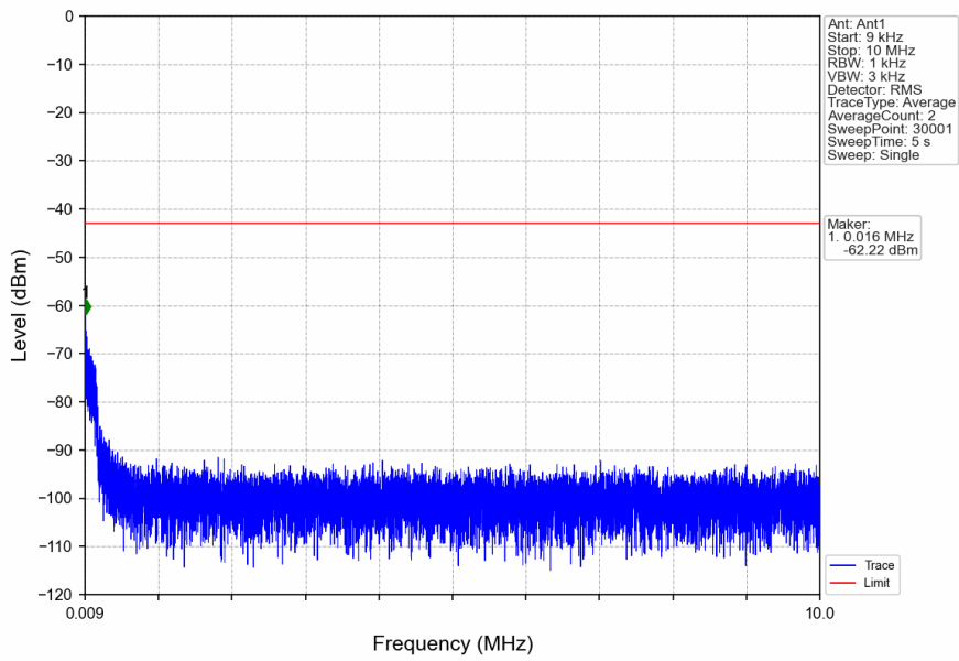
n5_15kHz_SISO_NTNV_5MHz_CP-OFDM QPSK_846.5MHz_Edge_1RB_Right
