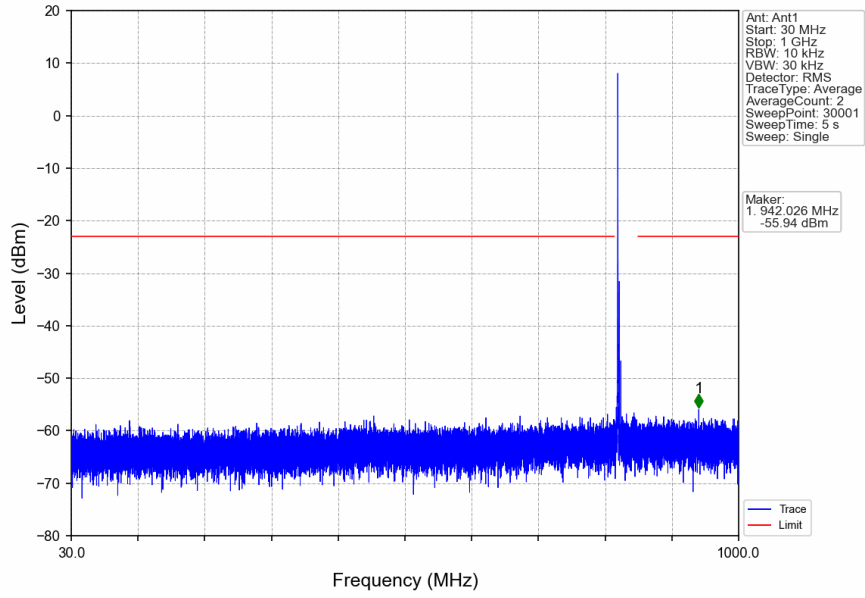
n5_15kHz_SISO_NTNV_5MHz_CP-OFDM QPSK_826.5MHz_Edge_1RB_Left
