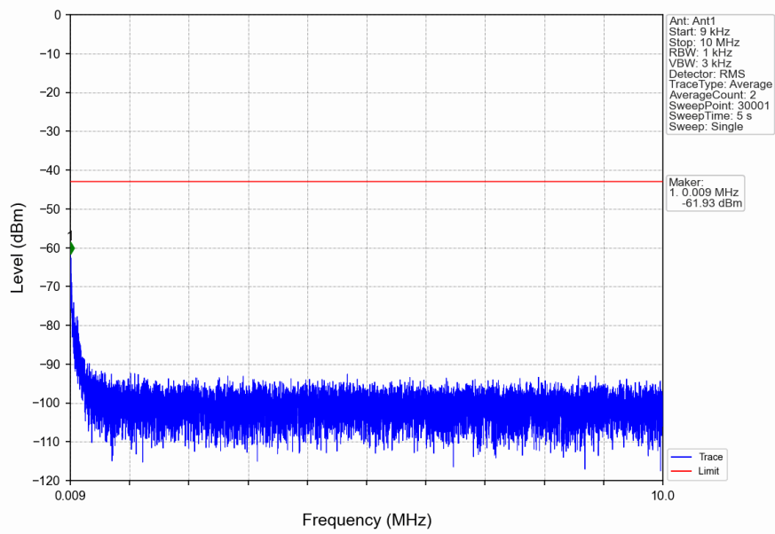
n2_15kHz_SISO_NTNV_15MHz_CP-OFDM QPSK_1902.5MHz_Edge_1RB_Right
