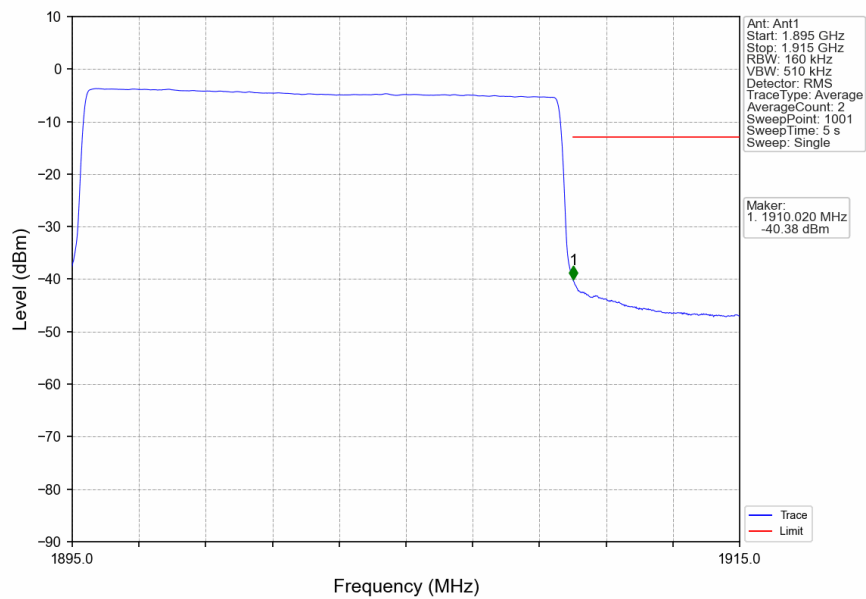
n2_15kHz_SISO_NTNV_15MHz_CP-OFDM QPSK_1902.5MHz_Outer_Full
