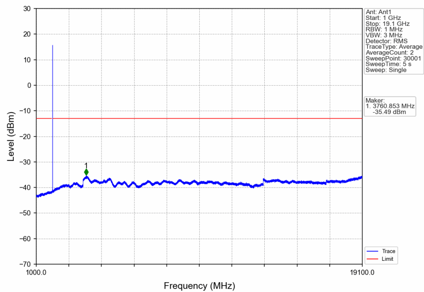
n2_15kHz_SISO_NTNV_15MHz_CP-OFDM QPSK_1902.5MHz_Inner_1RB_Right
