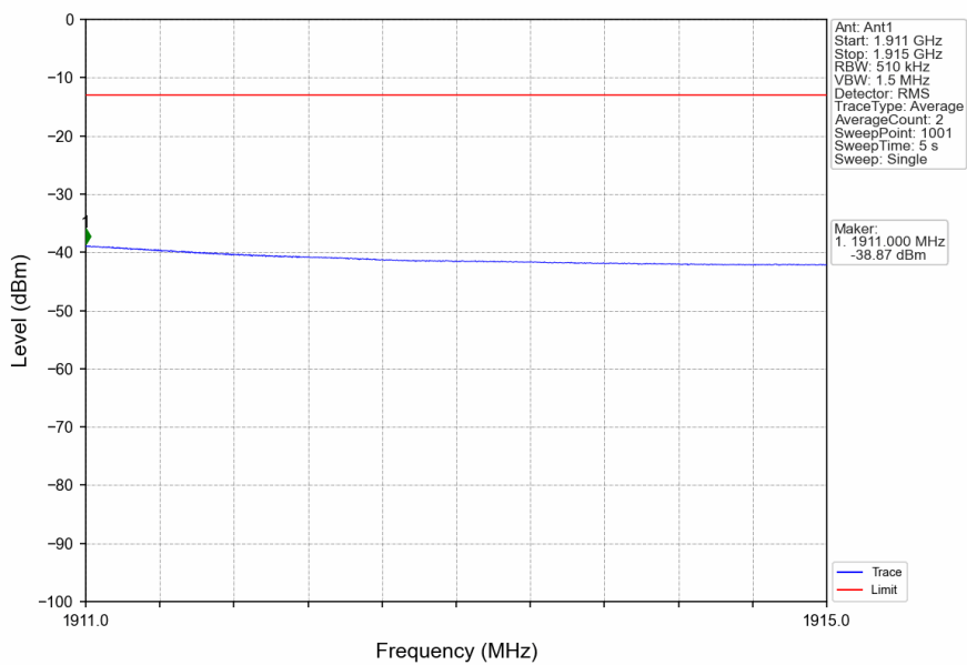
n2_15kHz_SISO_NTNV_15MHz_CP-OFDM QPSK_1902.5MHz_Outer_Full
