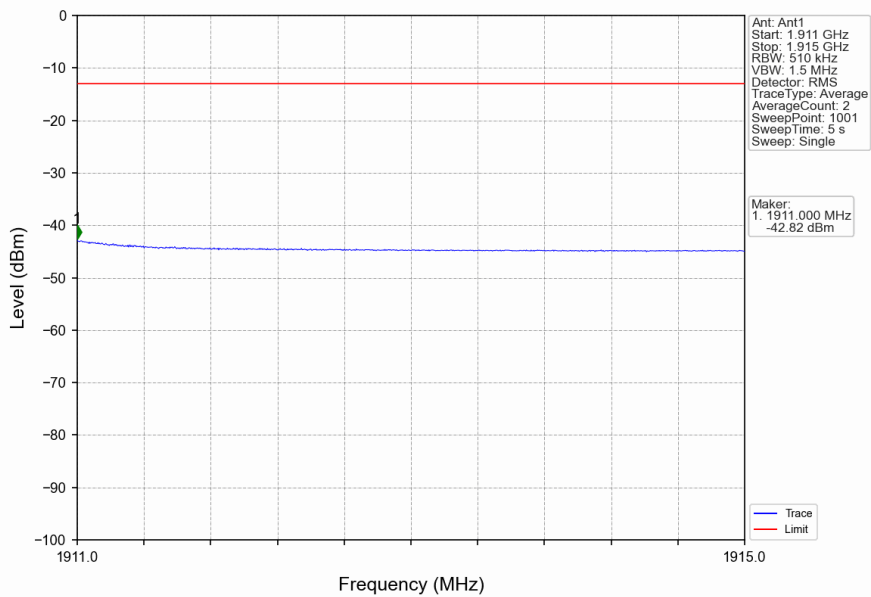
n2_15kHz_SISO_NTNV_15MHz_CP-OFDM QPSK_1902.5MHz_Edge_1RB_Right
