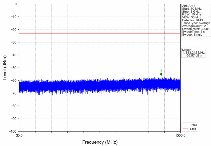
n2_15kHz_SISO_NTNV_15MHz_CP-OFDM QPSK_1902.5MHz_Inner_1RB_Right
