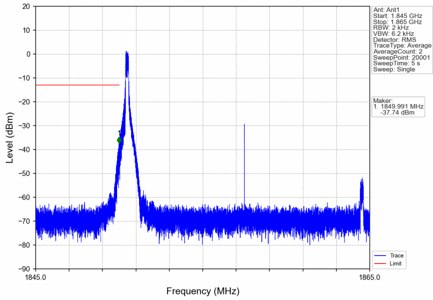
n2_15kHz_SISO_NTNV_15MHz_DFT-s-OFDM QPSK_1857.5MHz_Edge_1RB_Left
