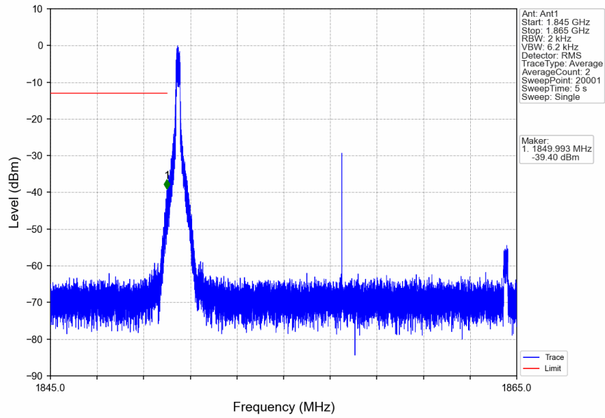
n2_15kHz_SISO_NTNV_15MHz_CP-OFDM QPSK_1857.5MHz_Edge_1RB_Left
