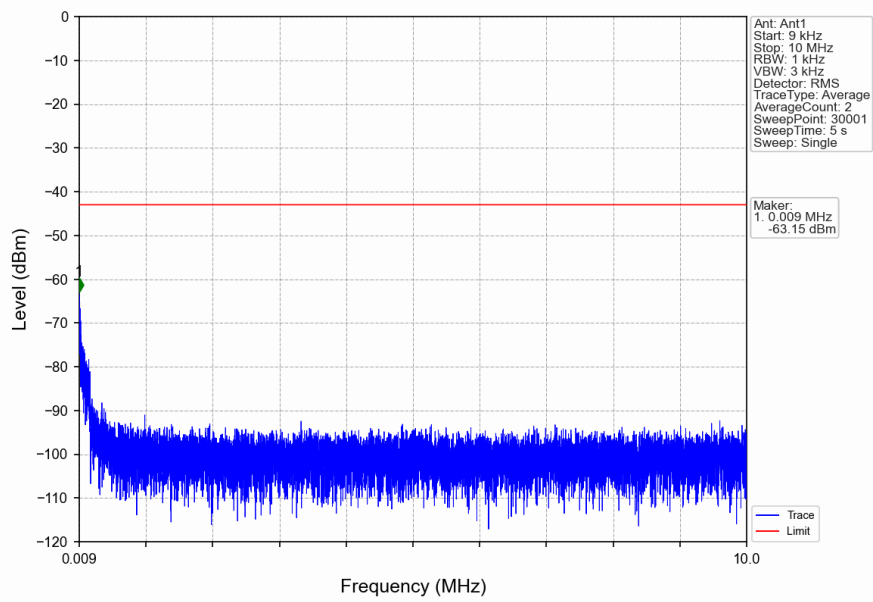
n2_15kHz_SISO_NTNV_15MHz_DFT-s-OFDM QPSK_1880MHz_Edge_1RB_Left
