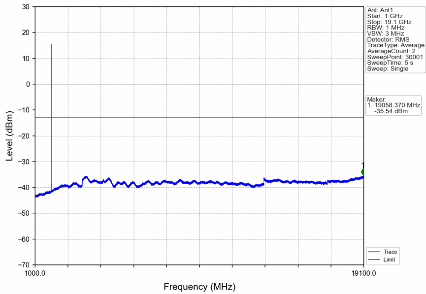
n2_15kHz_SISO_NTNV_15MHz_DFT-s-OFDM QPSK_1902.5MHz_Edge_1RB_Right
