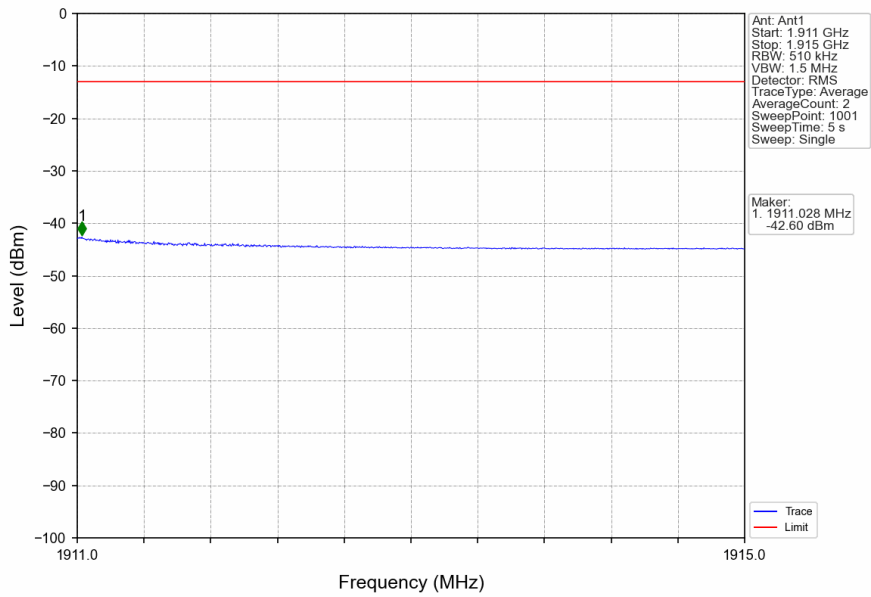
n2_15kHz_SISO_NTNV_15MHz_DFT-s-OFDM QPSK_1902.5MHz_Inner_1RB_Right
