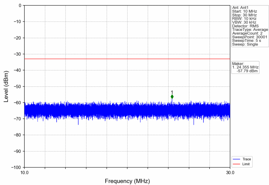
n2_15kHz_SISO_NTNV_15MHz_DFT-s-OFDM QPSK_1880MHz_Edge_1RB_Left
