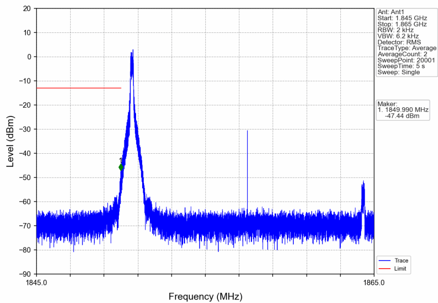
n2_15kHz_SISO_NTNV_15MHz_DFT-s-OFDM QPSK_1857.5MHz_Inner_1RB_Left
