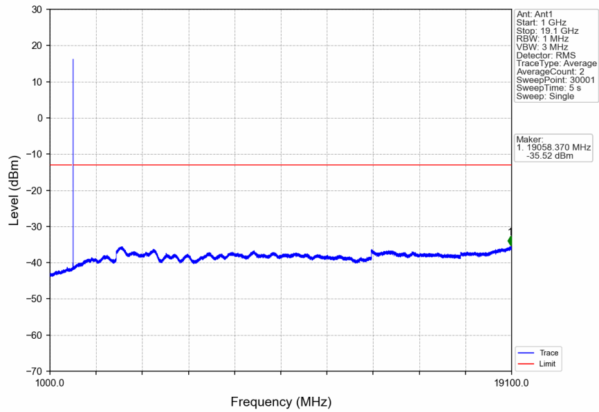
n2_15kHz_SISO_NTNV_15MHz_DFT-s-OFDM QPSK_1902.5MHz_Inner_1RB_Right
