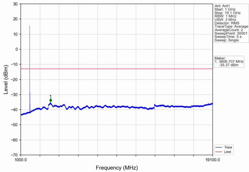
n2_15kHz_SISO_NTNV_15MHz_DFT-s-OFDM QPSK_1857.5MHz_Edge_1RB_Left
