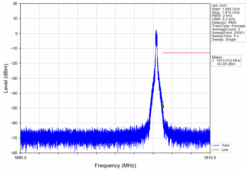
n2_15kHz_SISO_NTNV_15MHz_DFT-s-OFDM QPSK_1902.5MHz_Inner_1RB_Right
