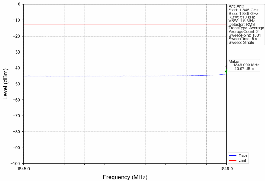
n2_15kHz_SISO_NTNV_15MHz_CP-OFDM QPSK_1857.5MHz_Edge_1RB_Left
