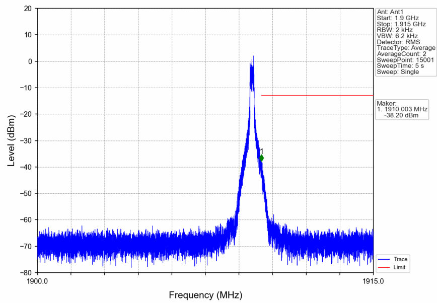
n2_15kHz_SISO_NTNV_10MHz_CP-OFDM QPSK_1905MHz_Edge_1RB_Right
