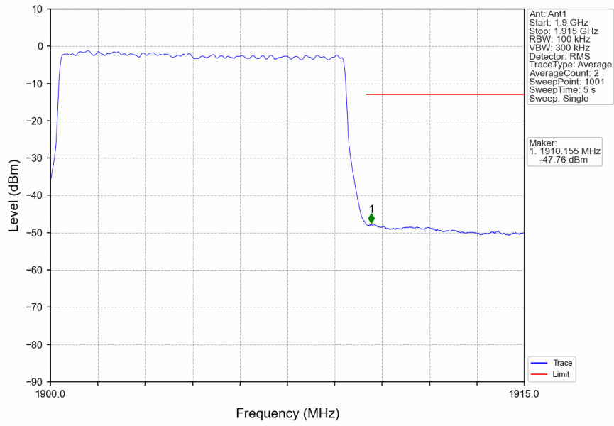
n2_15kHz_SISO_NTNV_10MHz_DFT-s-OFDM_QPSK_1905MHz_Outer_Full
