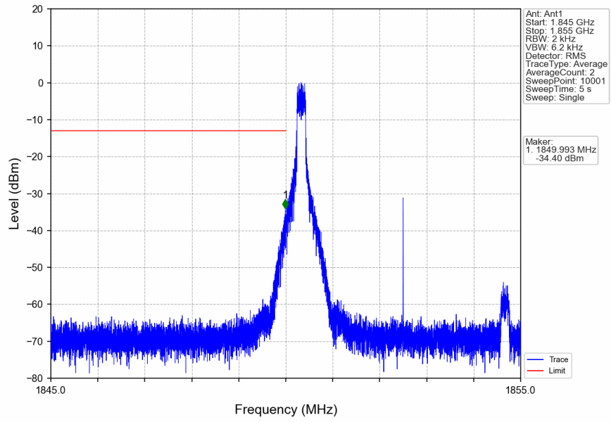
n2_15kHz_SISO_NTNV_5MHz_CP-OFDM QPSK_1852.5MHz_Edge_1RB_Left
