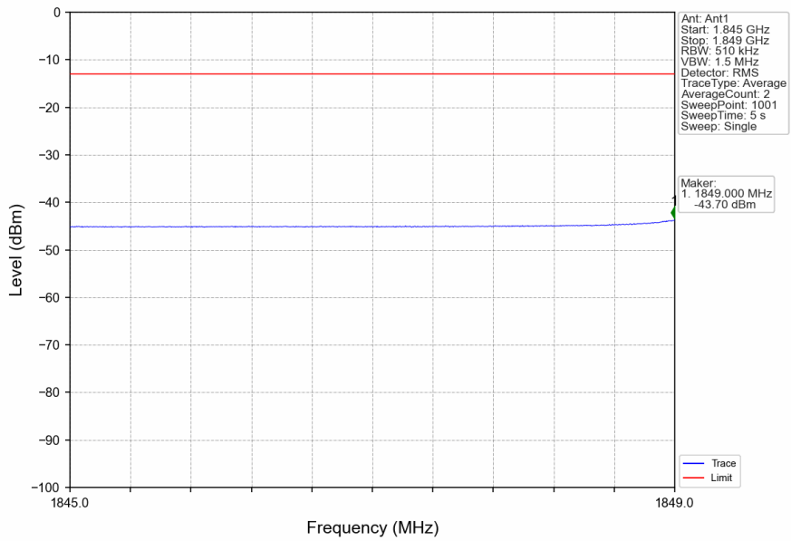
n2_15kHz_SISO_NTNV_5MHz_CP-OFDM QPSK_1852.5MHz_Edge_1RB_Left
