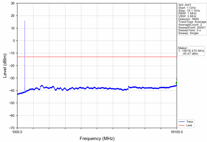
n2_15kHz_SISO_NTNV_5MHz_DFT-s-OFDM QPSK_1852.5MHz_Edge_1RB_Left
