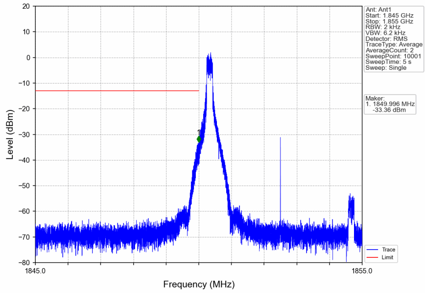
n2_15kHz_SISO_NTNV_5MHz_DFT-s-OFDM QPSK_1852.5MHz_Edge_1RB_Left
