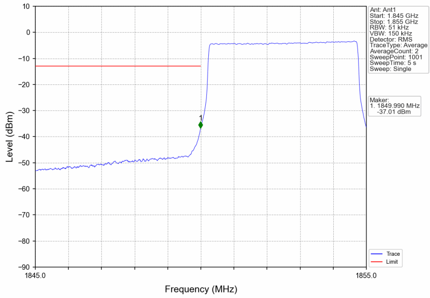
n2_15kHz_SISO_NTNV_5MHz_CP-OFDM QPSK_1852.5MHz_Outer_Full
