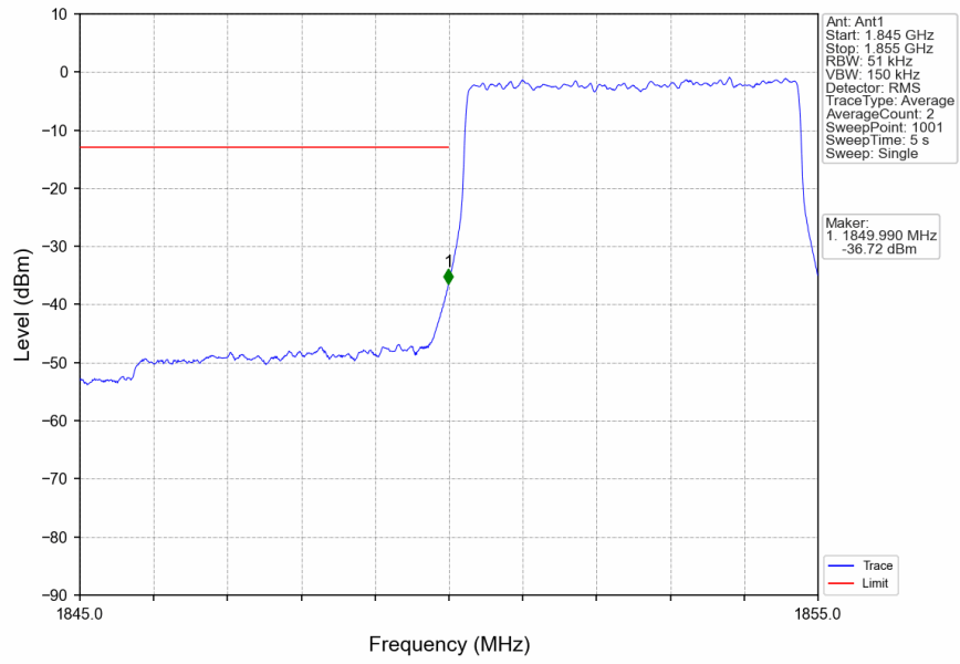
n2_15kHz_SISO_NTNV_5MHz_DFT-s-OFDM QPSK_1852.5MHz_Outer_Full
