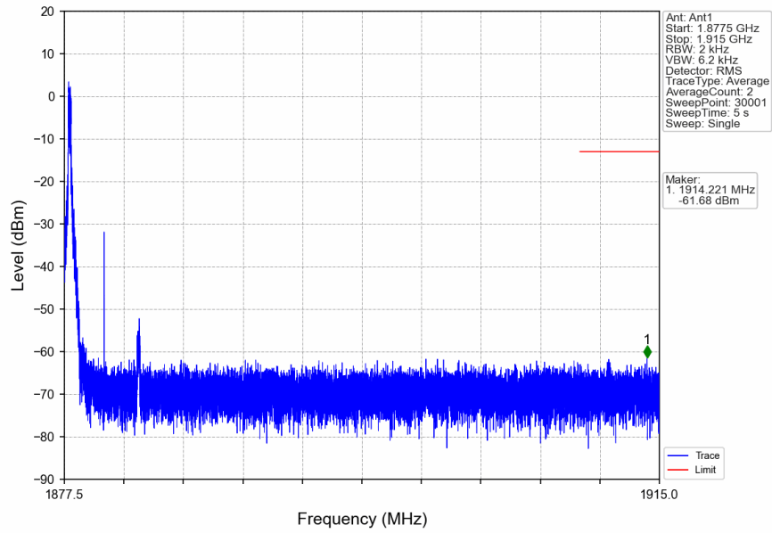
n2_15kHz_SISO_NTNV_5MHz_DFT-s-OFDM_QPSK_1880MHz_Edge_1RB_Left
