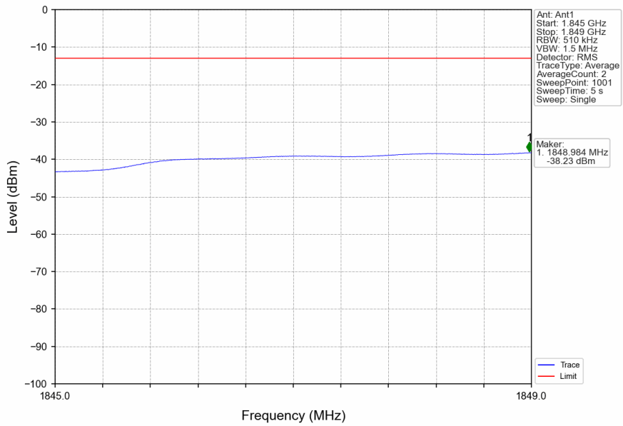
n2_15kHz_SISO_NTNV_5MHz_DFT-s-OFDM QPSK_1852.5MHz_Outer_Full
