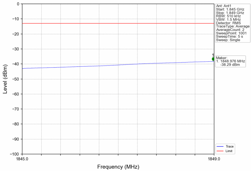
n2_15kHz_SISO_NTNV_5MHz_CP-OFDM QPSK_1852.5MHz_Outer_Full
