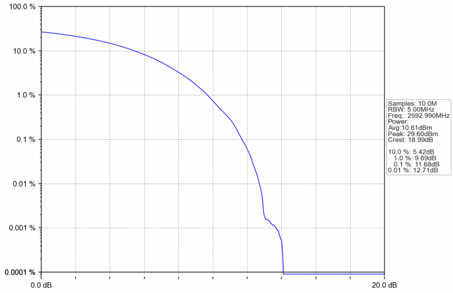
n41_30kHz_SISO_NTNV_40MHz_CP-OFDM 64 QAM_2592.99MHz_Outer_Full
