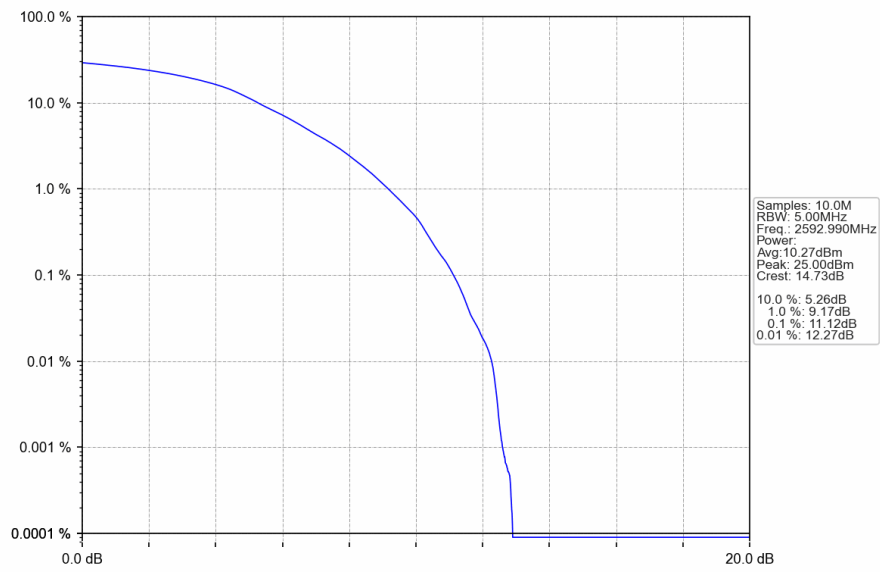
n41_30kHz_SISO_NTNV_60MHz_DFT-s-OFDM QPSK_2592.99MHz_Outer_Full
