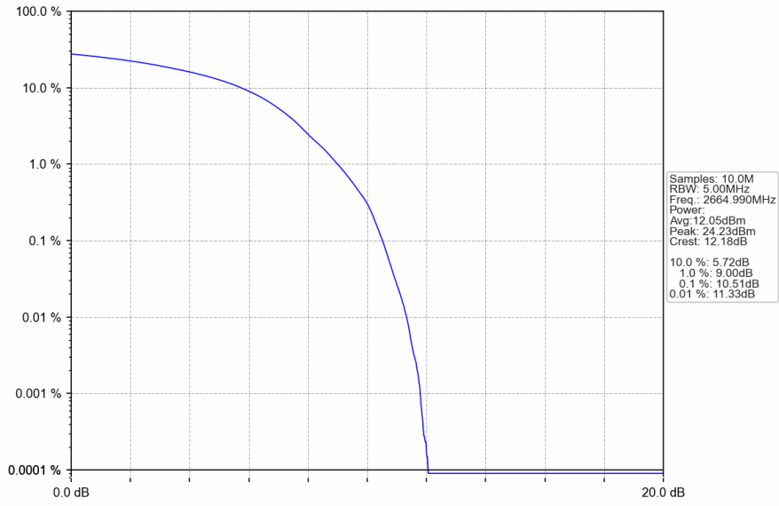
n41_30kHz_SISO_NTNV_50MHz_DFT-s-OFDM PI/2 BPSK_2664.99MHz_Outer_Full
