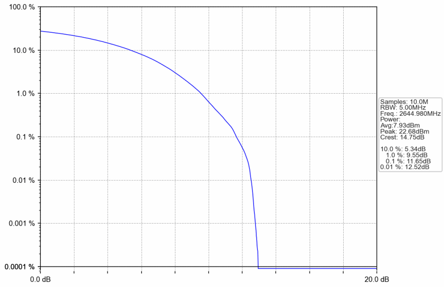
n41_30kHz_SISO_NTNV_90MHz_CP-OFDM 64 QAM_2644.98MHz_Outer_Full
