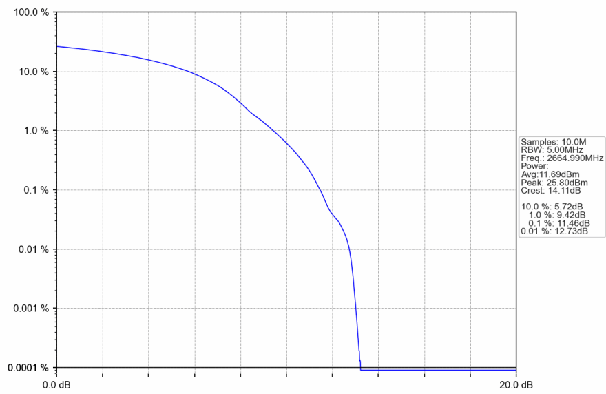
n41_30kHz_SISO_NTNV_50MHz_DFT-s-OFDM QPSK_2664.99MHz_Outer_Full
