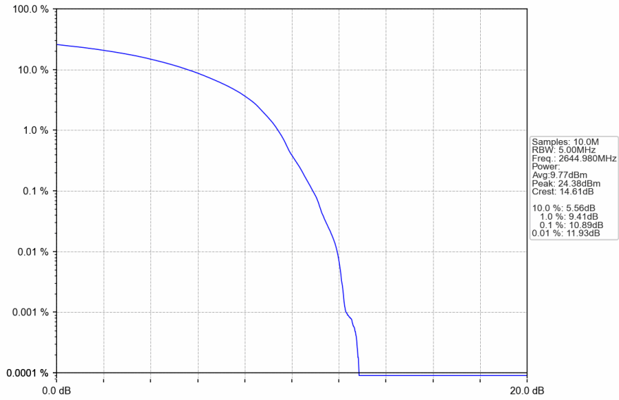
n41_30kHz_SISO_NTNV_90MHz_DFT-s-OFDM PI/2 BPSK_2644.98MHz_Outer_Full
