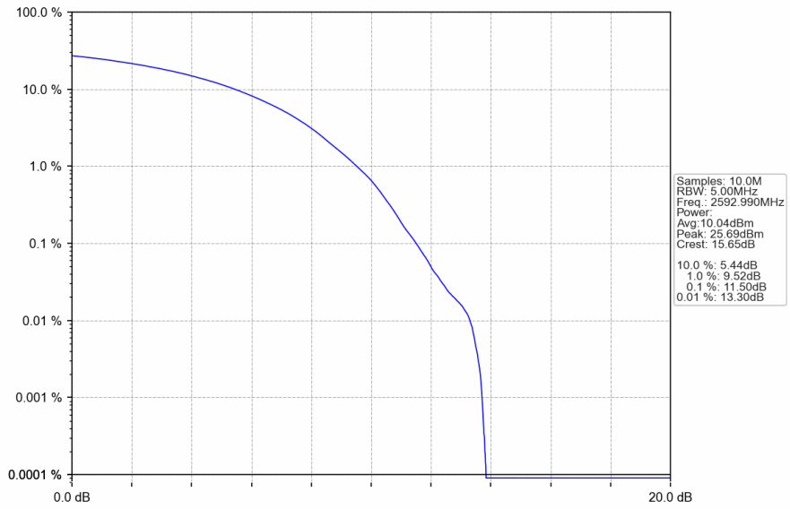
n41_30kHz_SISO_NTNV_50MHz_CP-OFDM 16 QAM_2592.99MHz_Outer_Full
