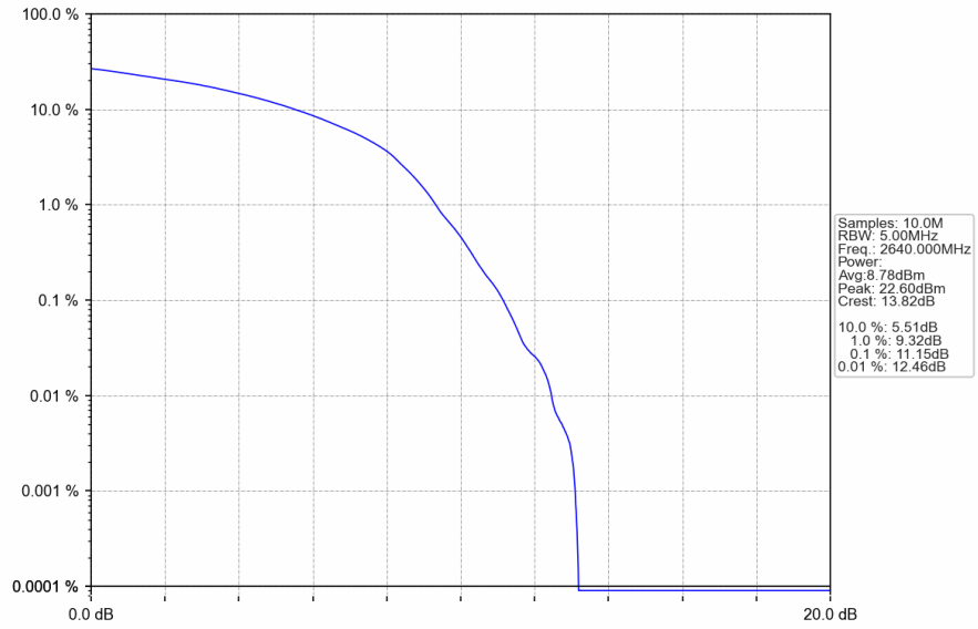
n41_30kHz_SISO_NTNV_100MHz_DFT-s-OFDM PI/2 BPSK_2640.00MHz_Outer_Full
