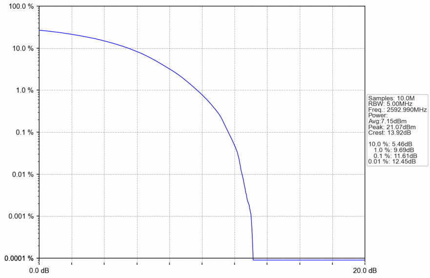
n41_30kHz_SISO_NTNV_80MHz_CP-OFDM 64 QAM_2592.99MHz_Outer_Full
