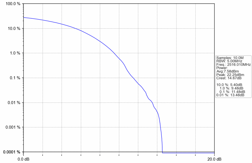
n41_30kHz_SISO_NTNV_40MHz_CP-OFDM 256 QAM 2516.01MHz_Outer_Full
