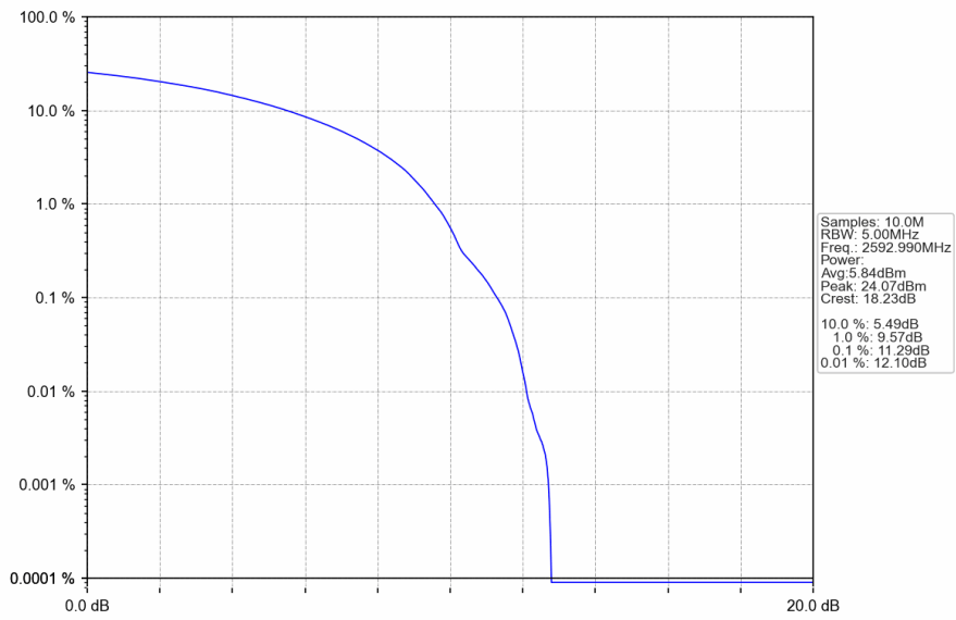
n41_30kHz_SISO_NTNV_90MHz_DFT-s-OFDM 256 QAM_2592.99MHz_Outer_Full
