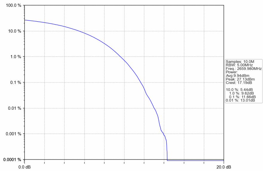
n41_30kHz_SISO_NTNV_60MHz_CP-OFDM QPSK_2659.98MHz_Outer_Full
