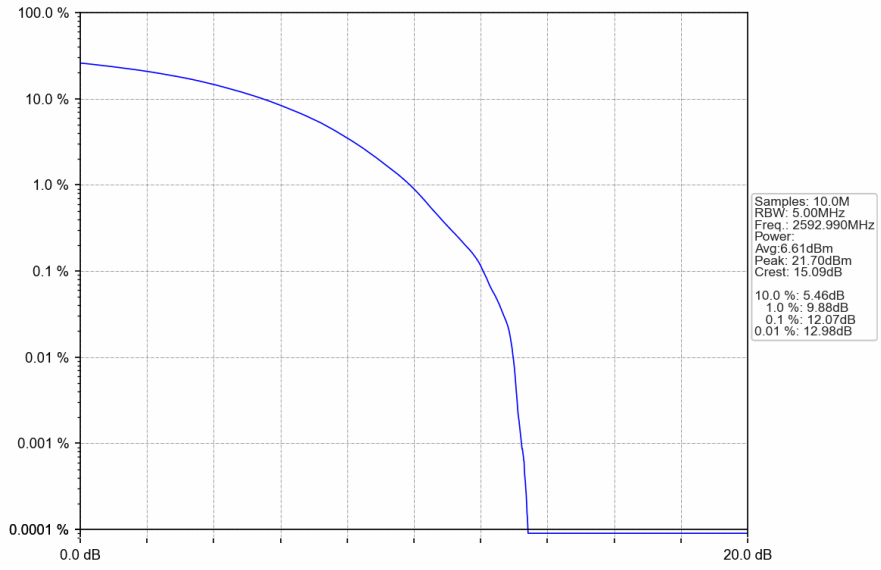
n41_30kHz_SISO_NTNV_90MHz_CP-OFDM 64 QAM_2592.99MHz_Outer_Full
