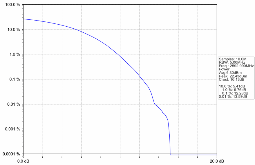
n41_30kHz_SISO_NTNV_50MHz_CP-OFDM 256 QAM 2592.99MHz_Outer_Full
