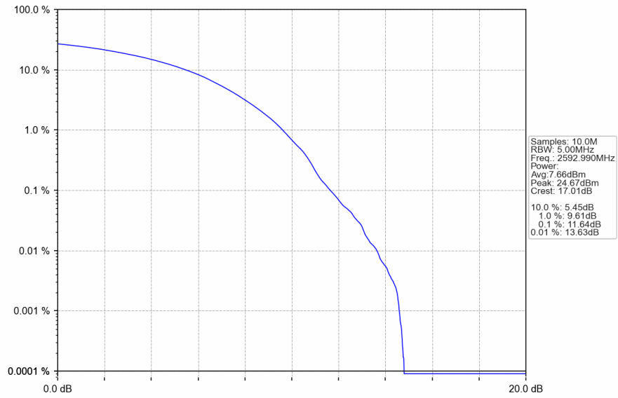
n41_30kHz_SISO_NTNV_40MHz_CP-OFDM 256 QAM 2592.99MHz_Outer_Full
