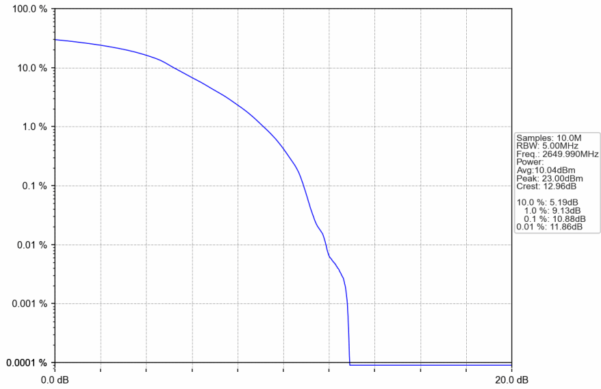
n41_30kHz_SISO_NTNV_80MHz_DFT-s-OFDM PI/2 BPSK_2649.99MHz_Outer_Full
