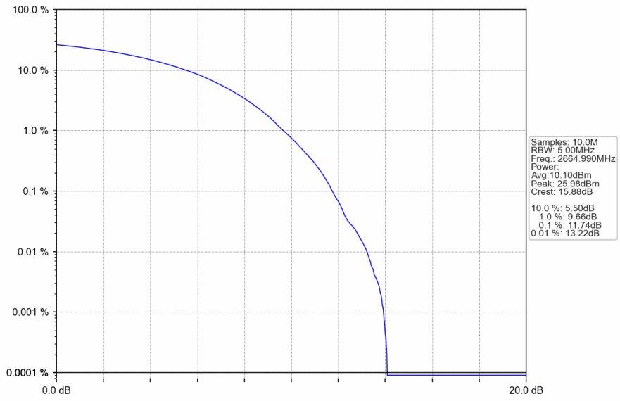
n41_30kHz_SISO_NTNV_50MHz_CP-OFDM 64 QAM_2664.99MHz_Outer_Full
