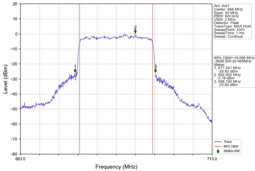
n71_15kHz_SISO_NTNV_20MHz_CP-OFDM 64 QAM_688MHz_Outer_Full
