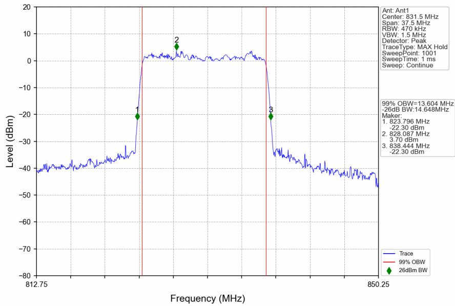
n5_15kHz_SISO_NTNV_15MHz_DFT-s-OFDM QPSK_831.5MHz_Outer_Full
