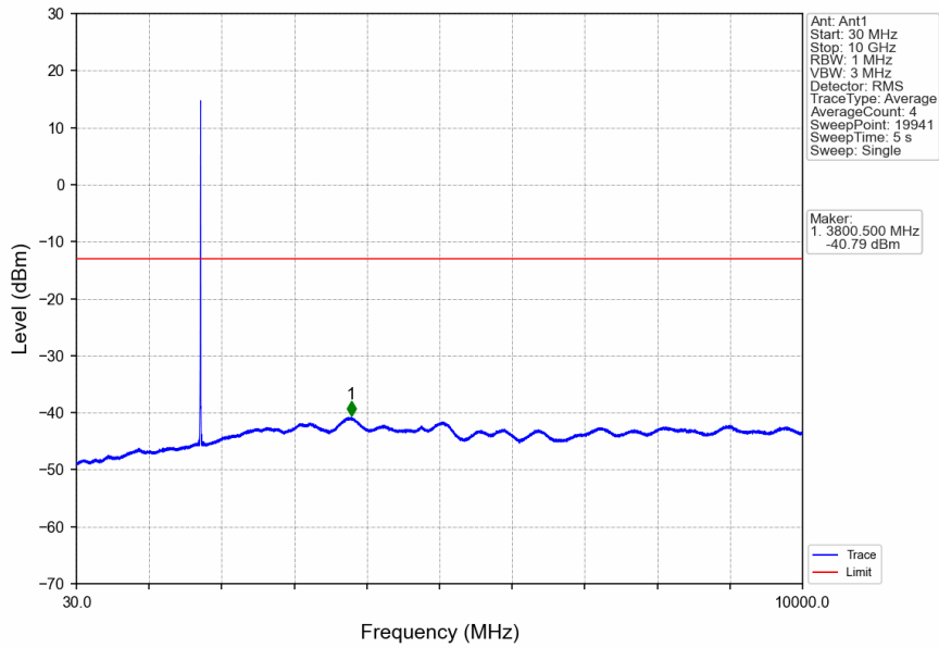
Band4_HSDPA_MCH_1732.6MHz_Subtest 1_NTNV
