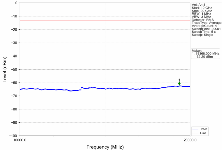
Band4_RMC_MCH_1732.6MHz_12.2kbps RMC_NTNV
