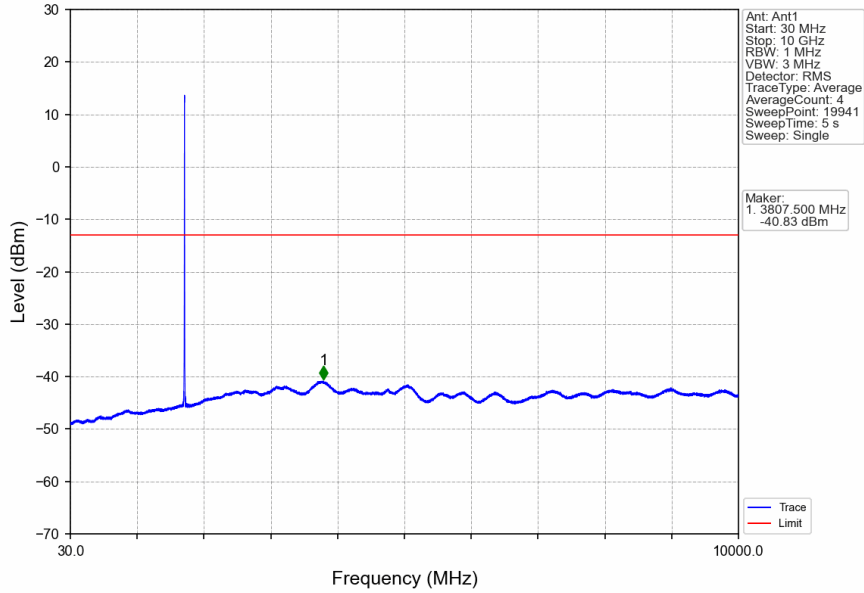
Band4_HSUPA_MCH_1732.6MHz_Subtest 1_NTNV
