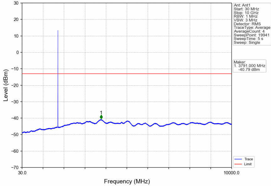
Band4_RMC_MCH_1732.6MHz_12.2kbps RMC_NTNV
