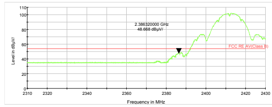
802.11b-Channel 1 Average
