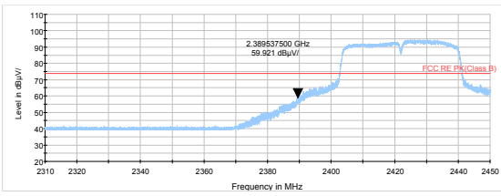
802.11n HT40 -Channel 3 Peak
