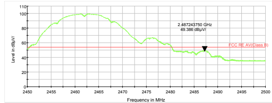
802.11b-Channel 11 Average
