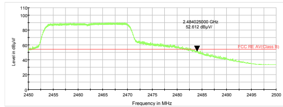
802.11g-Channel 11 Average
