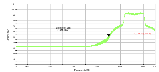
802.11g-Channel 1 Average
