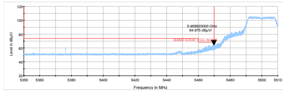
802.11n HT20-Channel 100: Average
