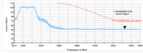
802.11n HT20-Channel 165: Peak
