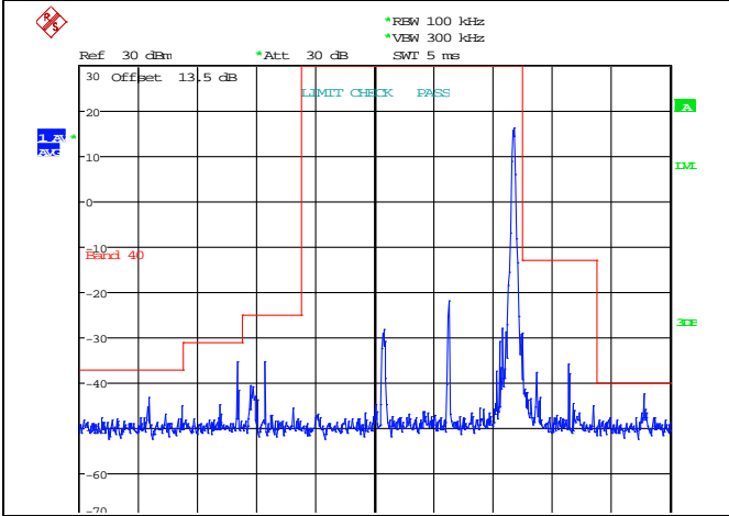
QPSK Low channel-1 RB offset max
