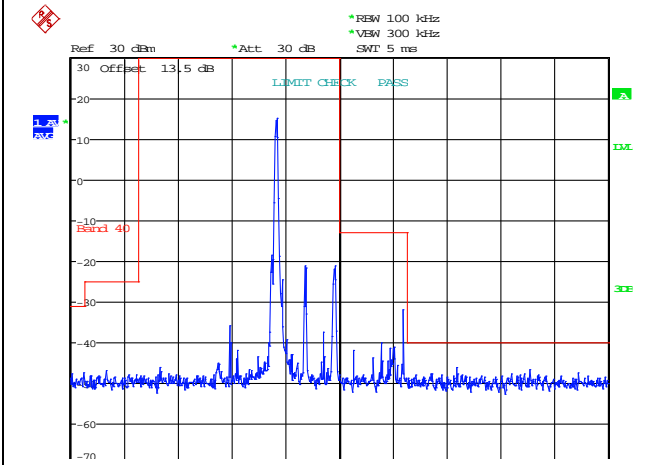
QPSK High channel-25 RB offset 0
