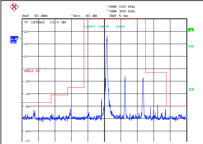
QPSK Low channel-50 RB offset 0
