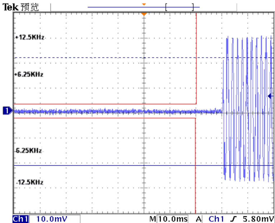
Transmitter Frequency Behaviour @ 12.5 KHz Channel Separation-----On – Off
