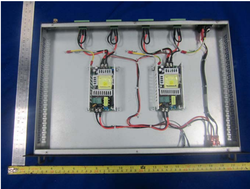
EUT –Power Supply Uncover View
