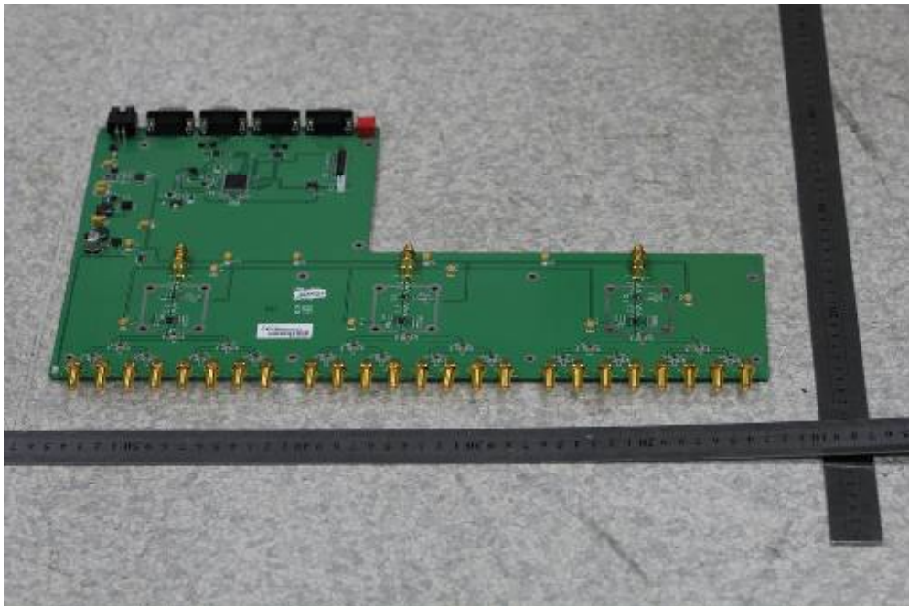
EUT – DIU Main Board Top View
