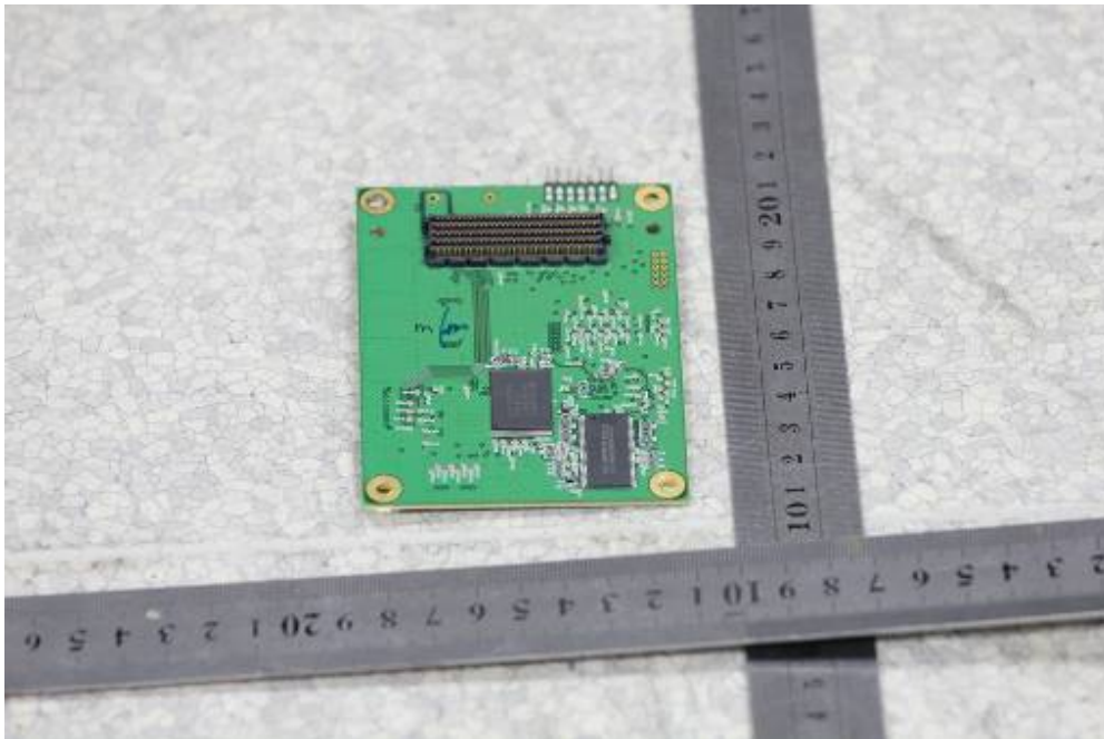
EUT – CHU CHB-MB Bottom View
