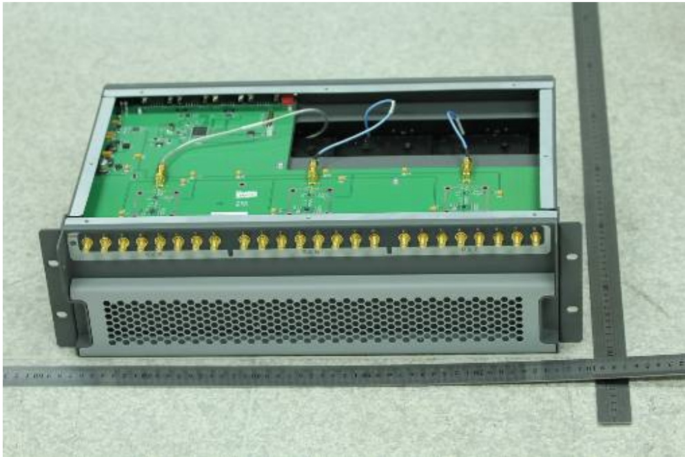
EUT – DIU Cover off View
