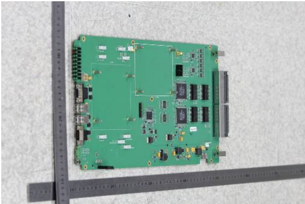
EUT – BSCU Main Board Top View
