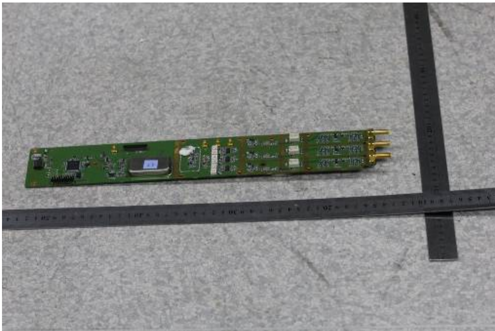
EUT – CHU RX Board Top View
