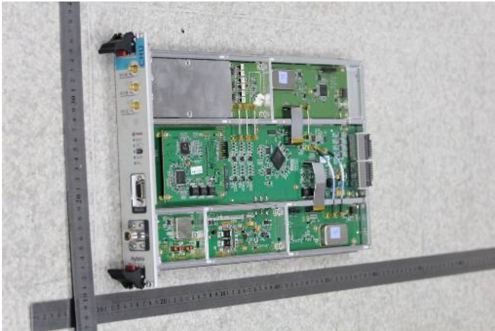
EUT – CHU Cover off View
