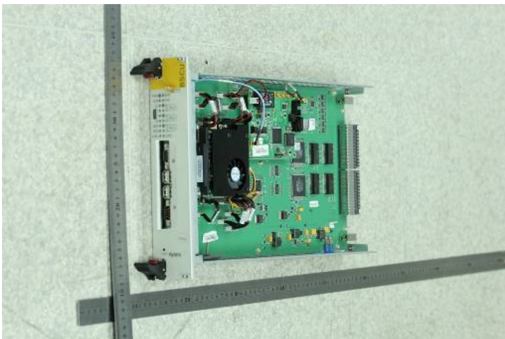
EUT – BSCU Cover off View
