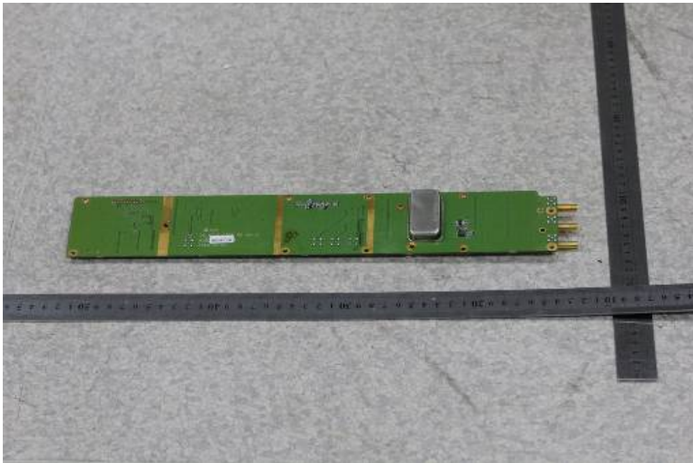
EUT – CHU RX Board Bottom View
