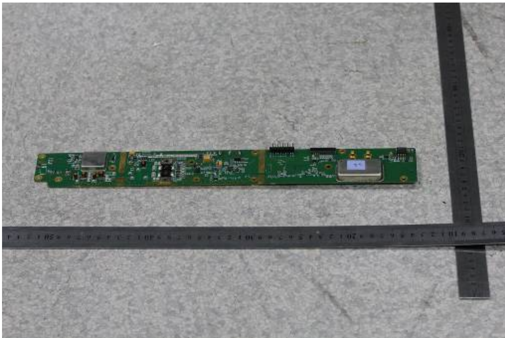
EUT – CHU TX Board Top View
