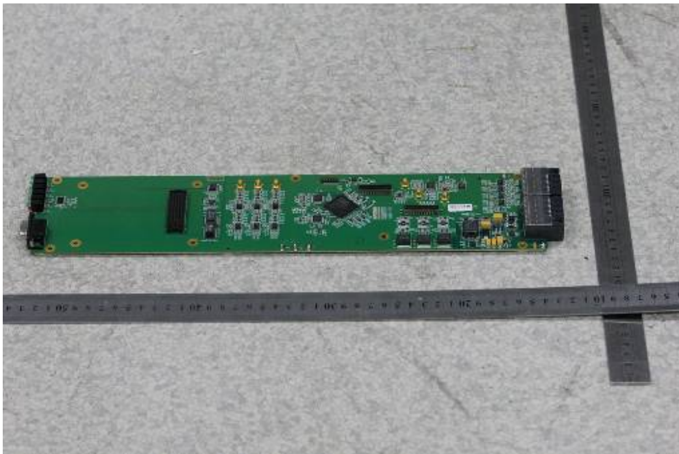
EUT – CHU CHB Top View
