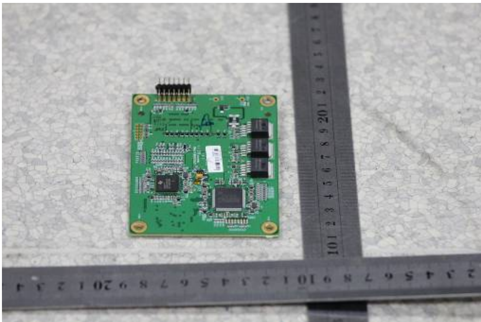
EUT – CHU CHB-MB Top View
