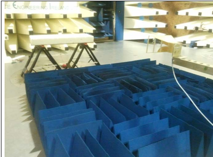
Fig 4 Test setup
