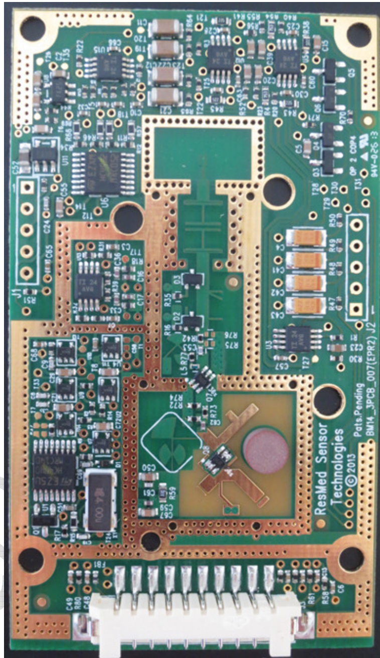
Fig.2 PCB Top Side with metal work removed
