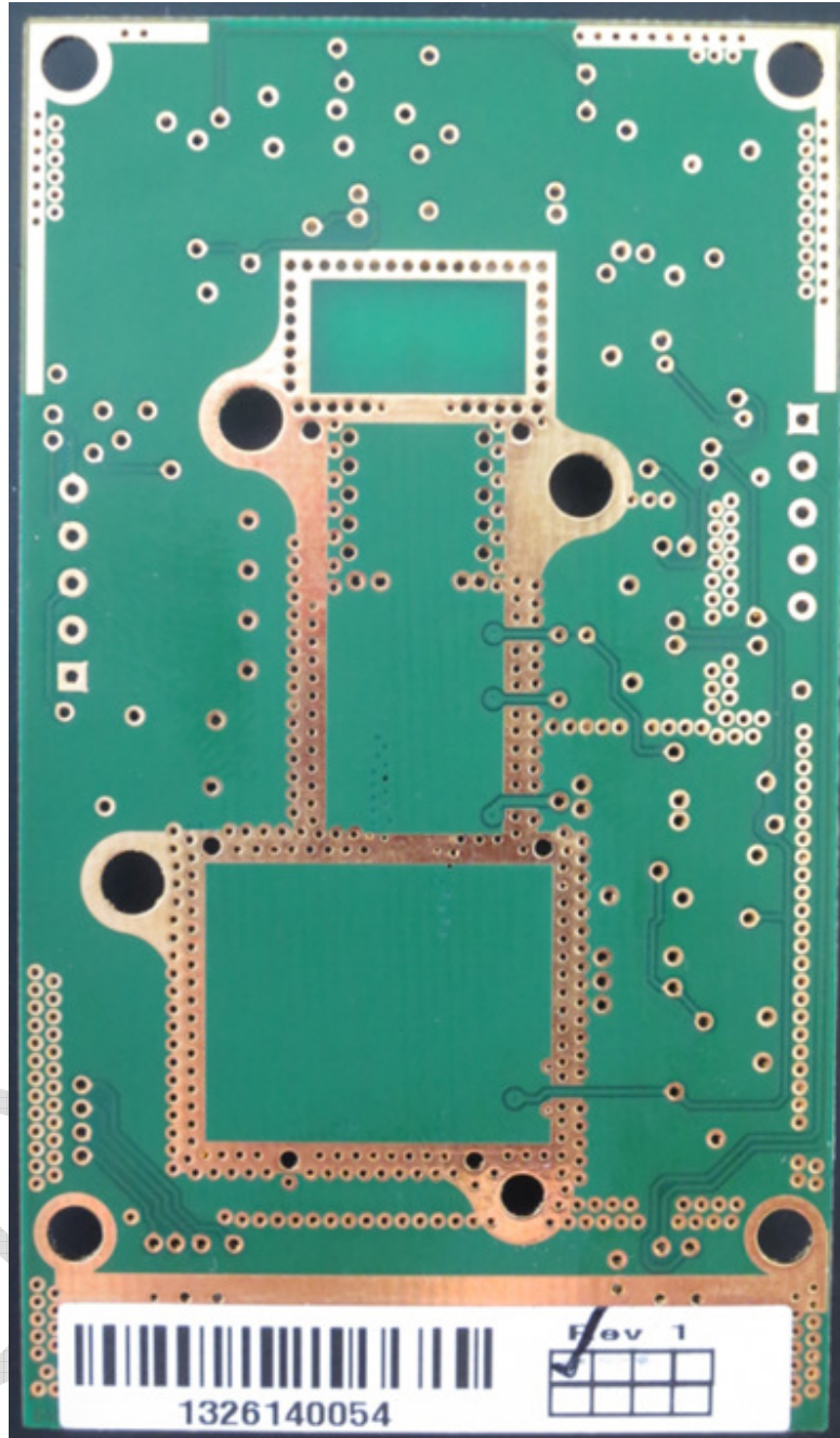
Fig.4 PCB Bottom Side with metal work removed
