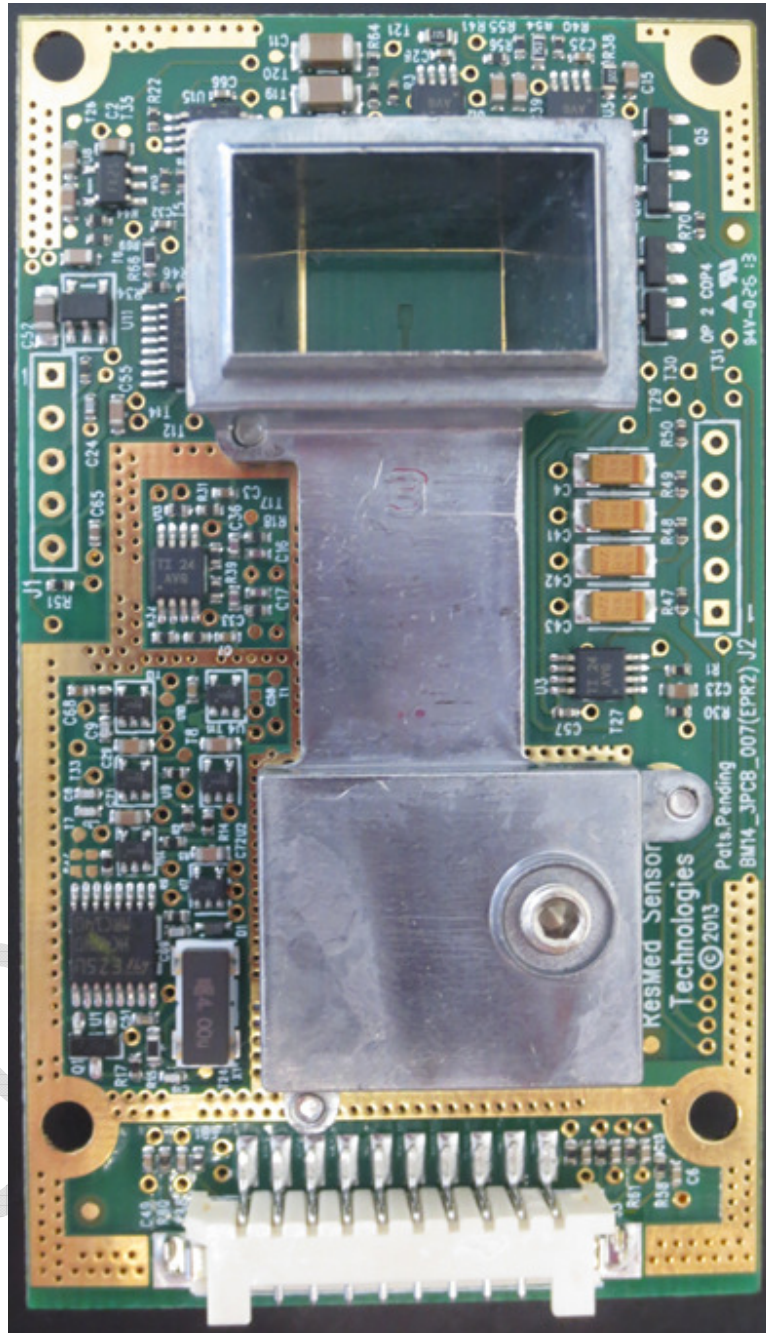
Fig.1 PCB Top Side with metal work and Horn antenna
