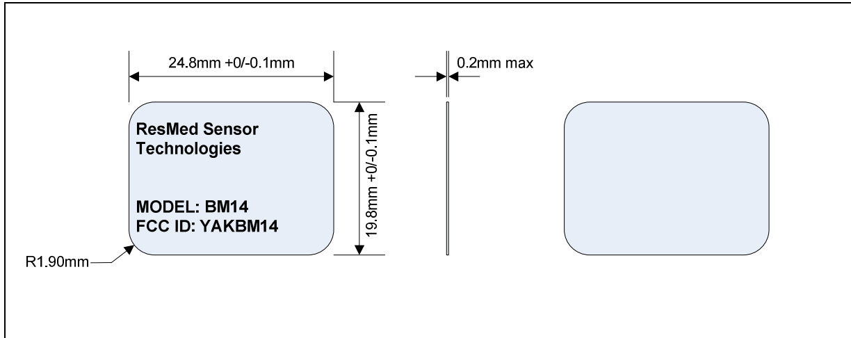
FCC Label drawing:
