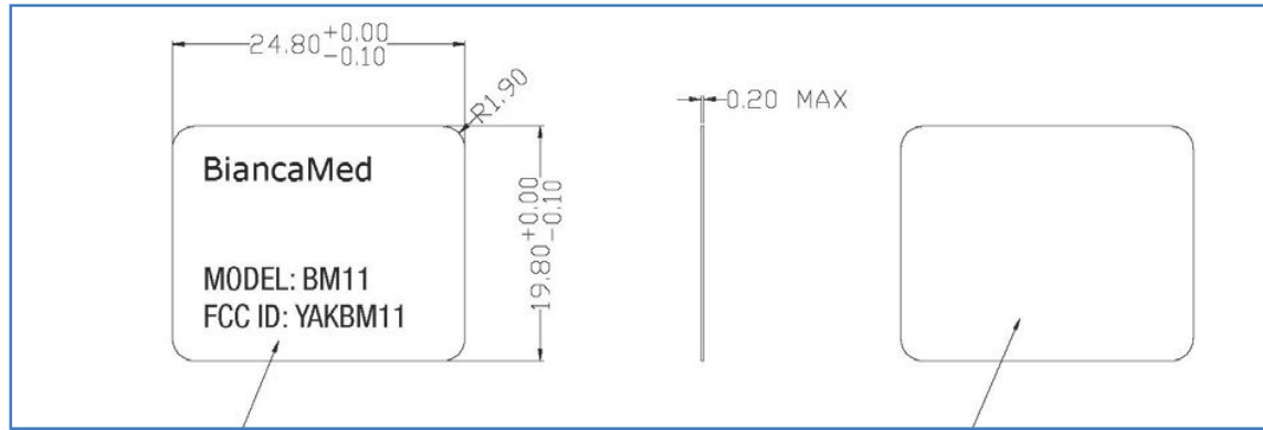
FCC Label drawing:
