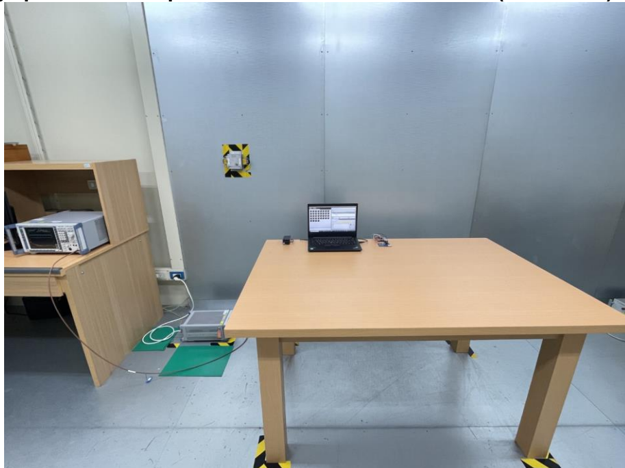
Photograph 8: Test Setup for Mains Conducted Emissions (Front View)
