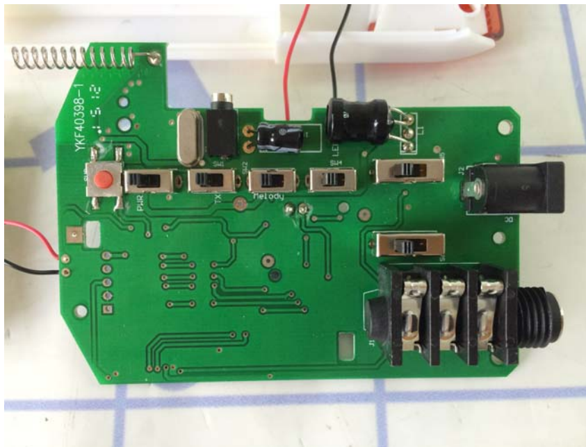
PCB 2 side 2
