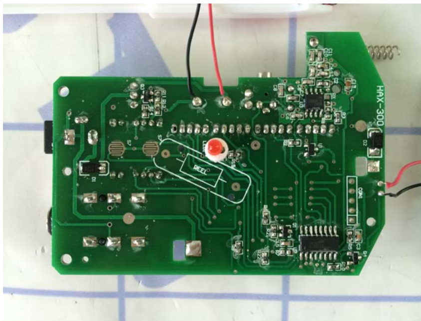
PCB 2 side 1
