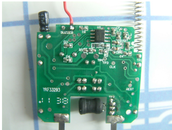
PCB layout-1
