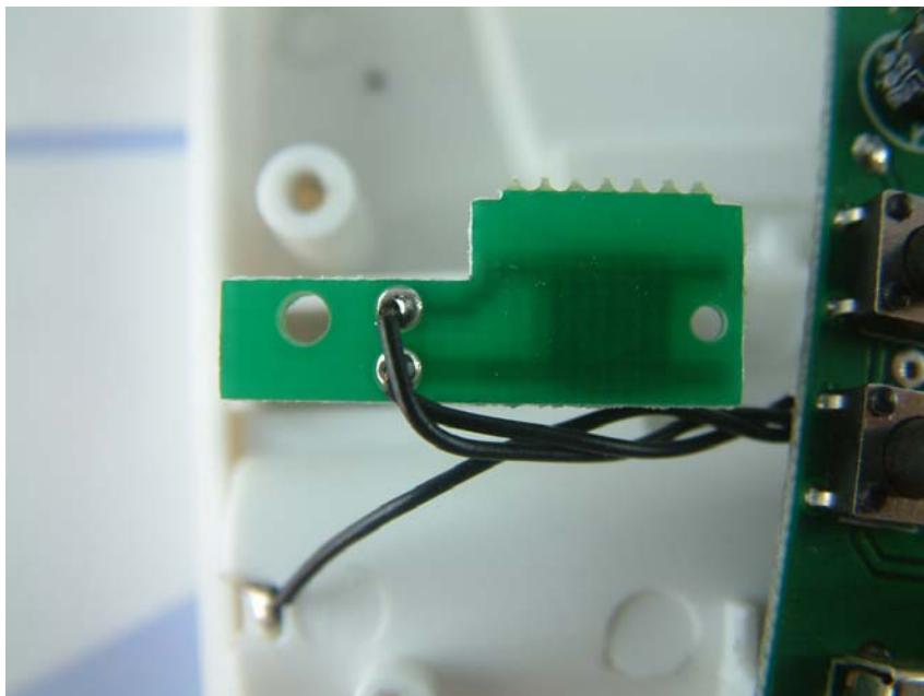
PCB 3 side 2
