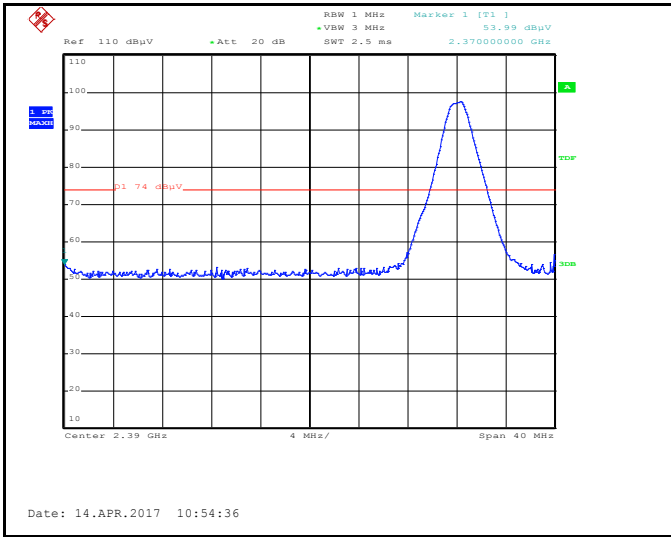
Band Edge, Left Side (Peak - Horizontal)
