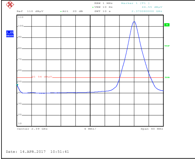
Band Edge, Left Side (Average - Vertical)
