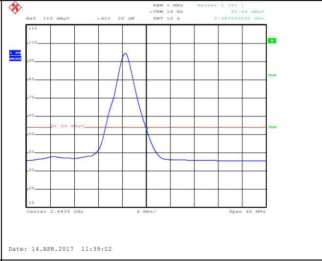
Band Edge, Right Side (Average - Vertical)
