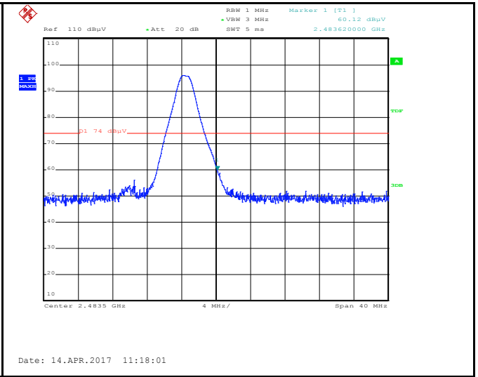
Band Edge, Right Side (Peak - Horizontal)
