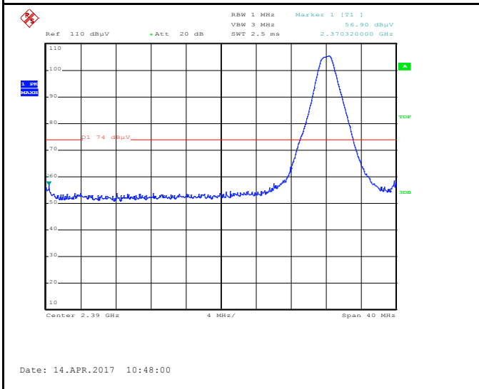
Band Edge, Left Side (Peak - Vertical)
