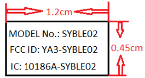
Silk screen
